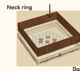
Fig. 12b. Neck ring over the base.
