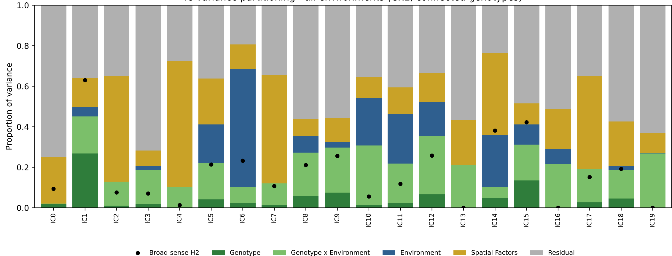
IC variance partitioning - all environments (GxE, connected genotypes)
