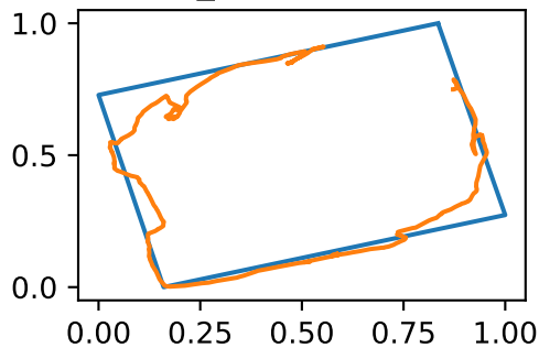
ave_100 prediction
