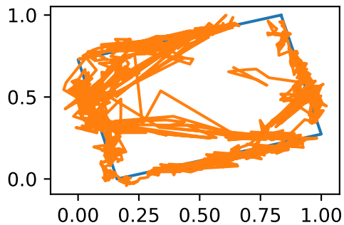
raw prediction
