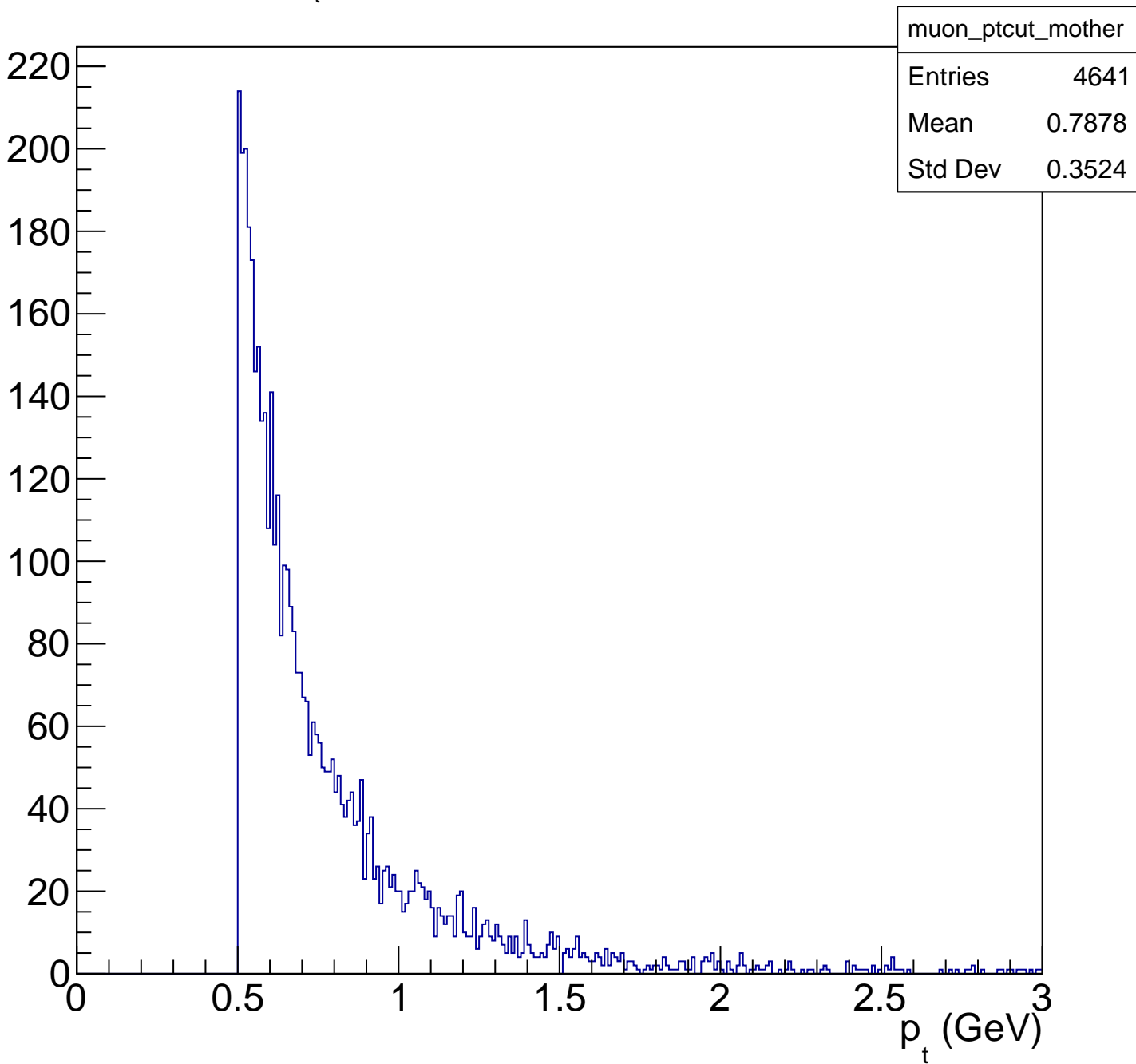
\mu^- and \mu^+ p_t distribution after cuts (with same mother ( \eta ))
