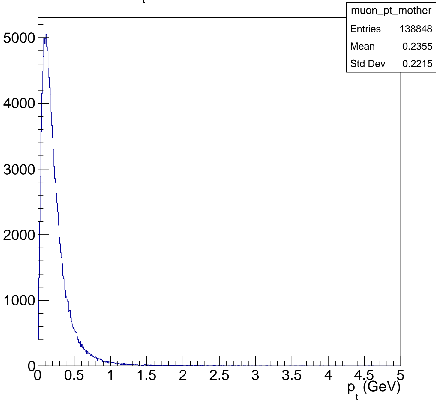
\mu^- and \mu^+ p_t distribution with same mother ( \eta )
