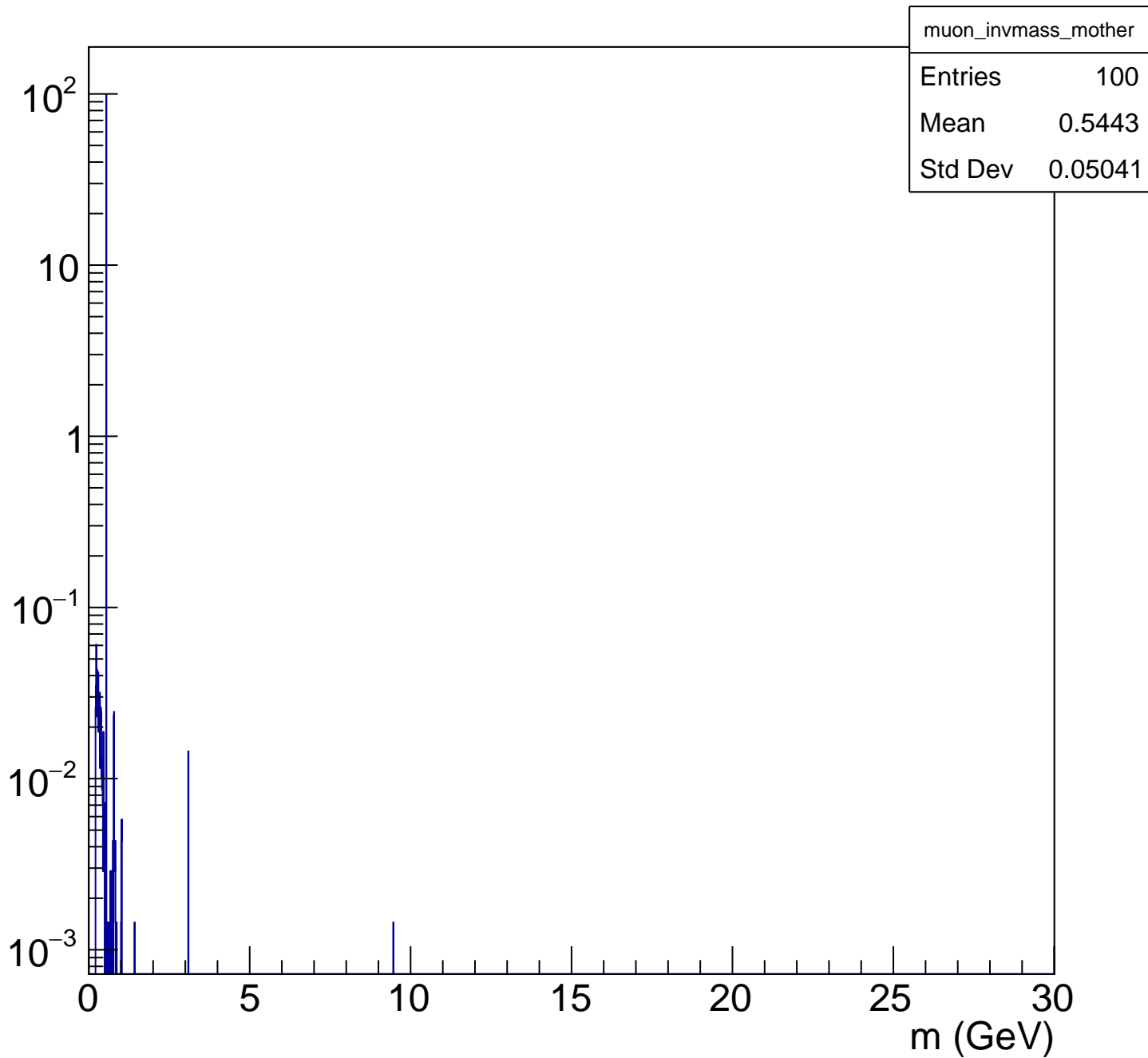
Reconstructed muon pair invariant mass with same mother
