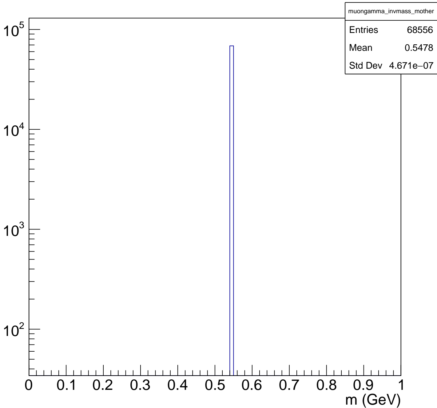
Reconstructed muon pair + \gamma invariant mass with same mother
