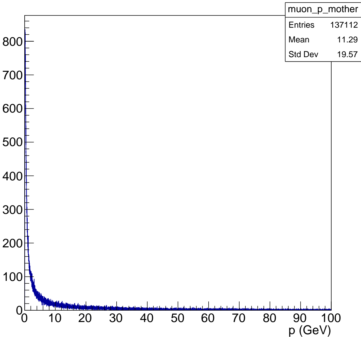
\mu^- and \mu^+ p distribution with same mother ( \eta )
