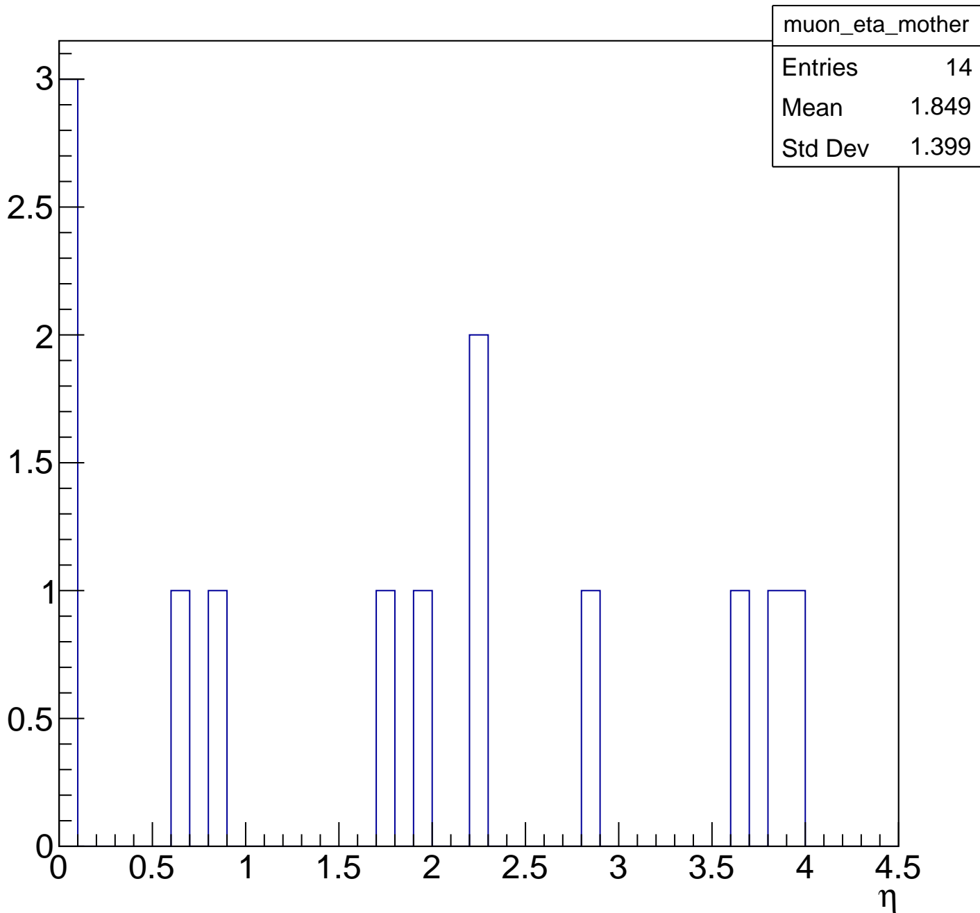
\mu^- and \mu^+ pseudorapidity distribution with same mother ( \eta )
