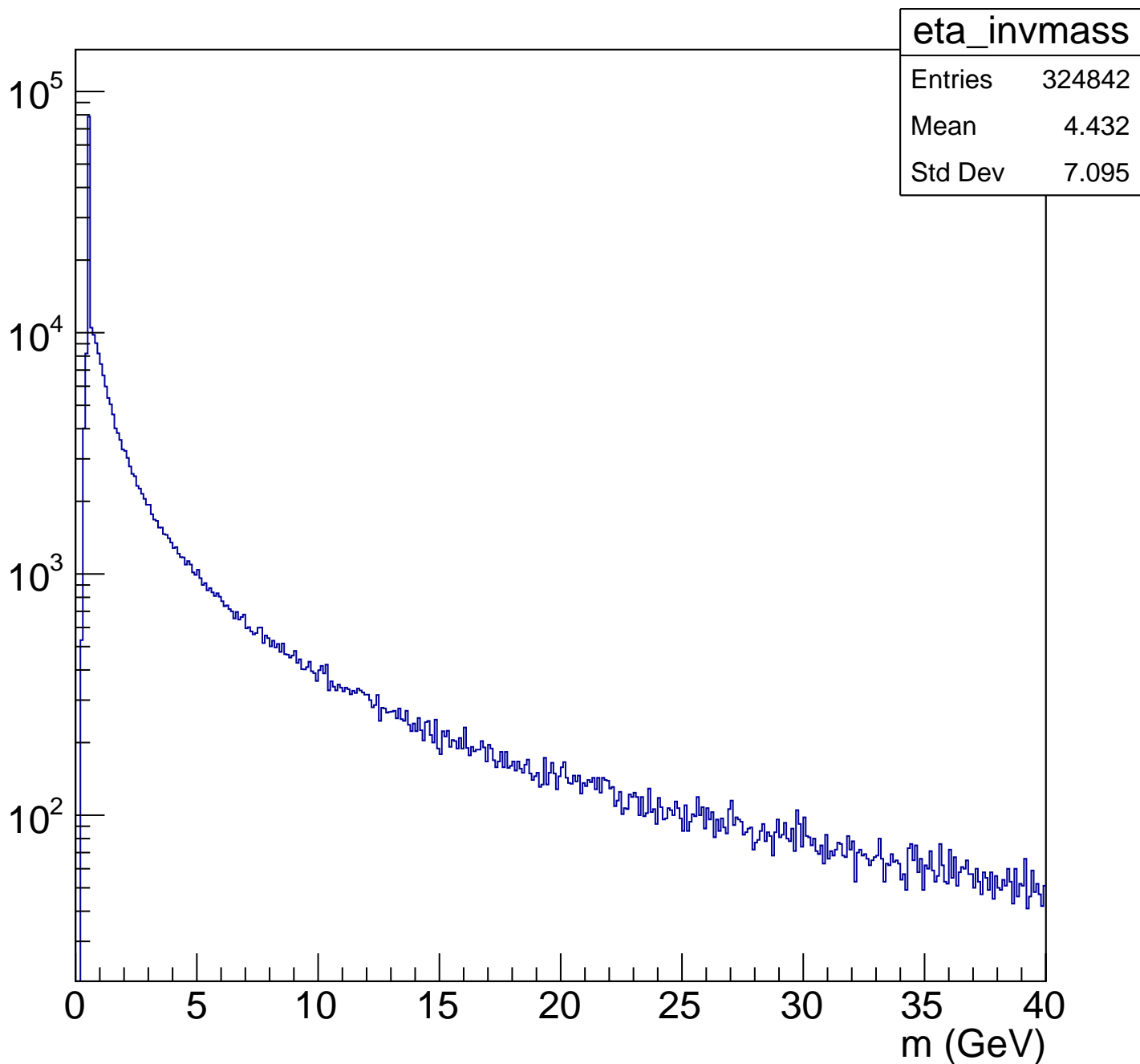
Reconstructed eta invariant mass from muon pairs and gamma
