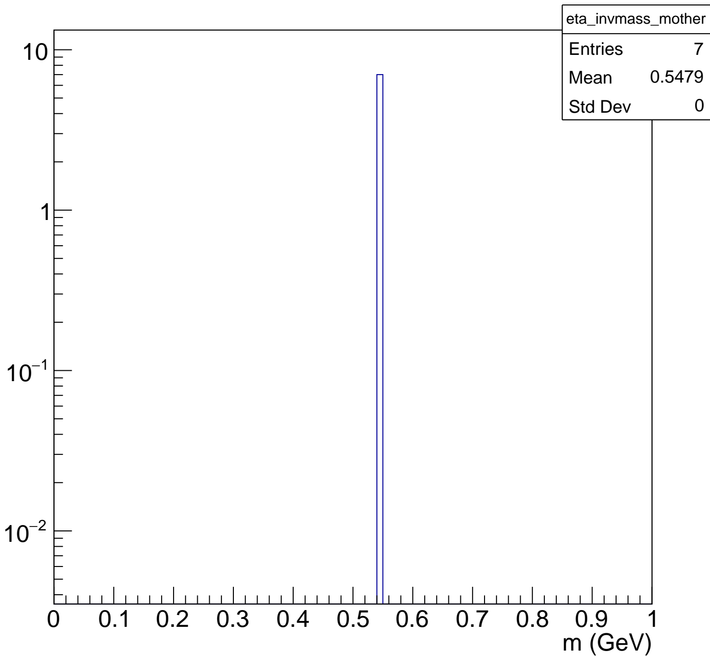
Reconstructed \eta invariant mass from muon pairs with same mother
