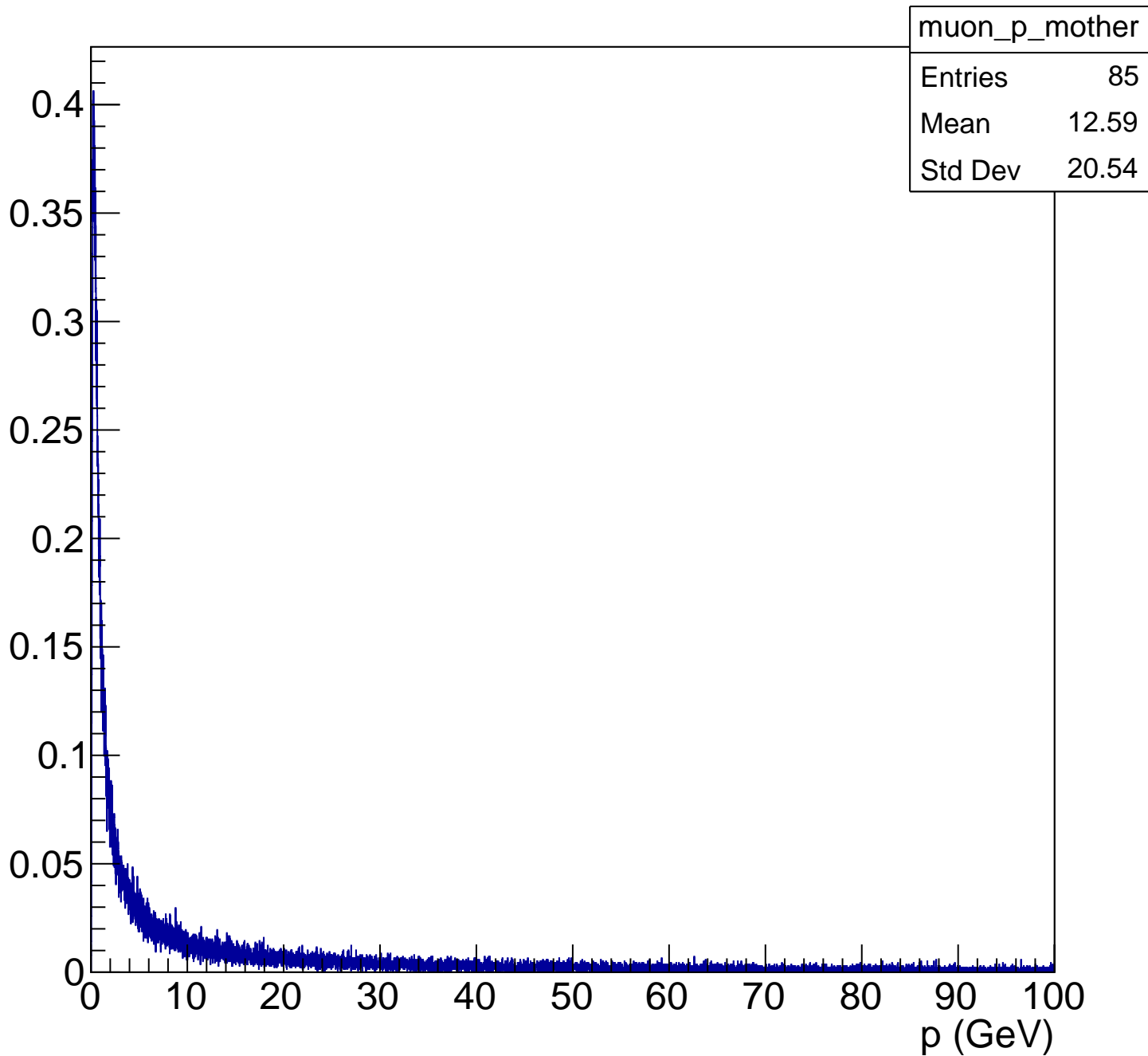
\mu^- and \mu^+ p distribution with same mother ( \eta )
