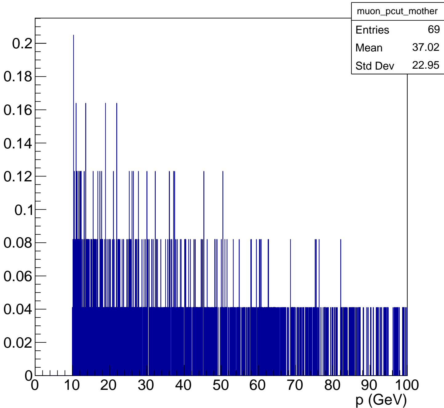
\mu^- and \mu^+ p distribution after cuts (with same mother ( \eta ))
