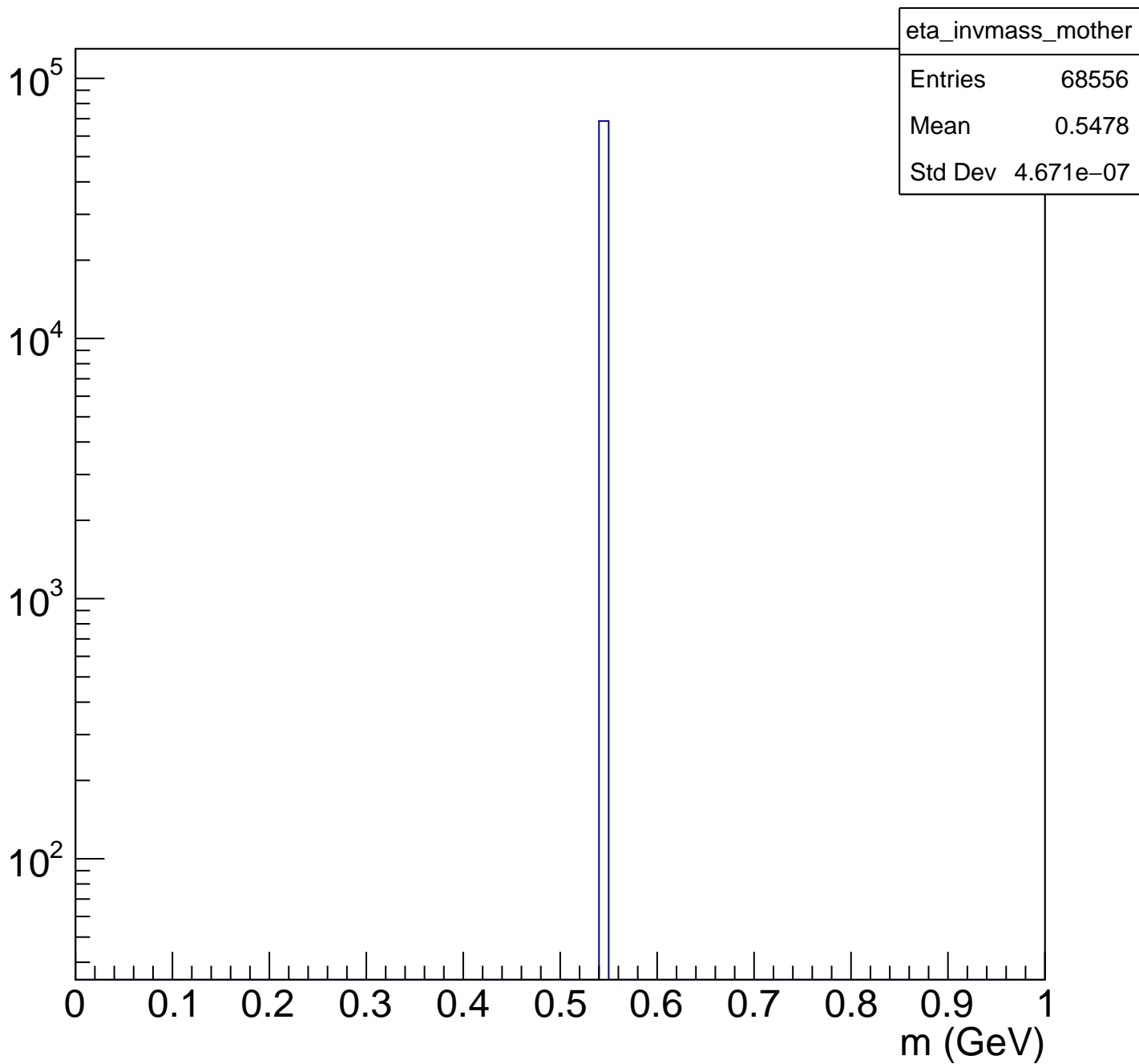
Reconstructed invariant mass from muon pairs + \gamma with same mother ( \eta )
