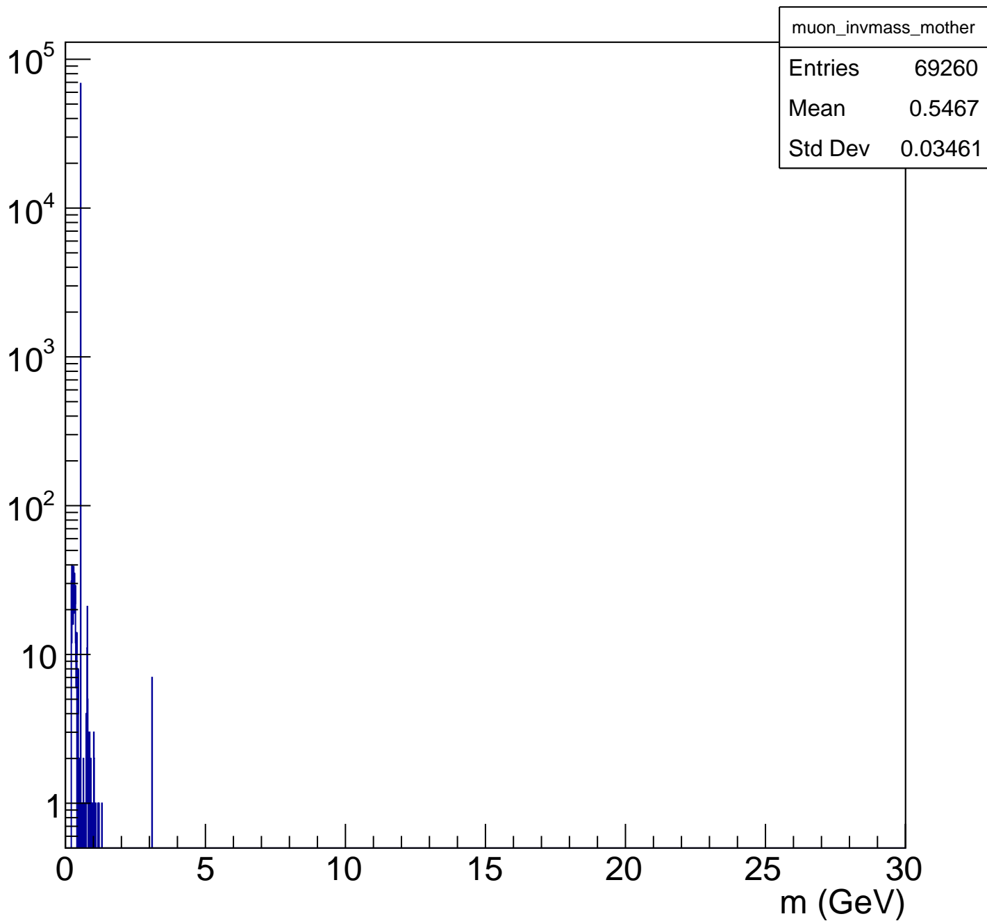
Reconstructed muon pair invariant mass with same mother
