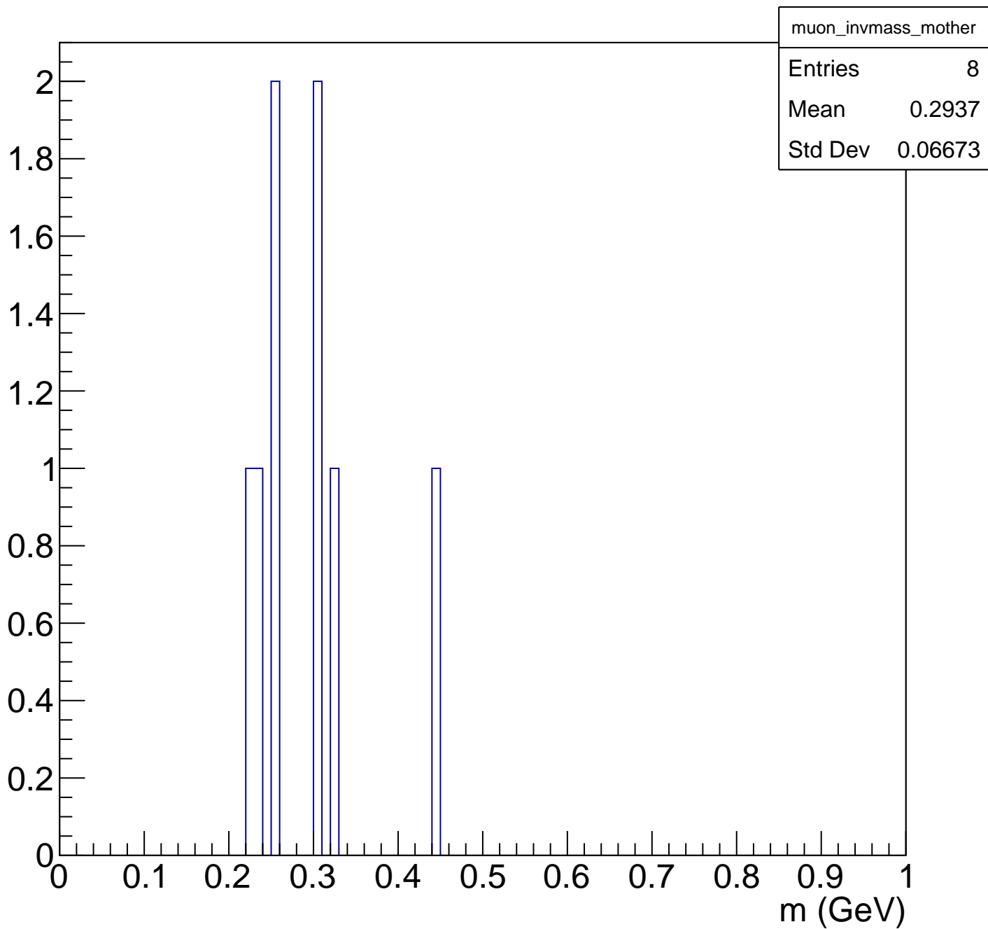
Reconstructed muon pair invariant mass with same mother( \eta )
