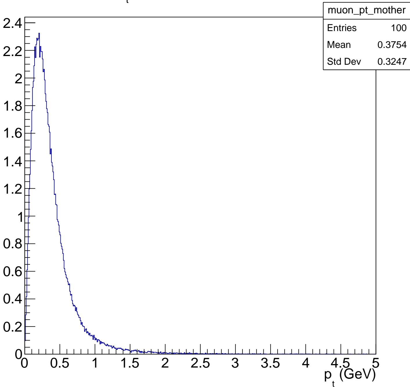
\mu^- and \mu^+ p_t distribution with same mother ( \eta )
