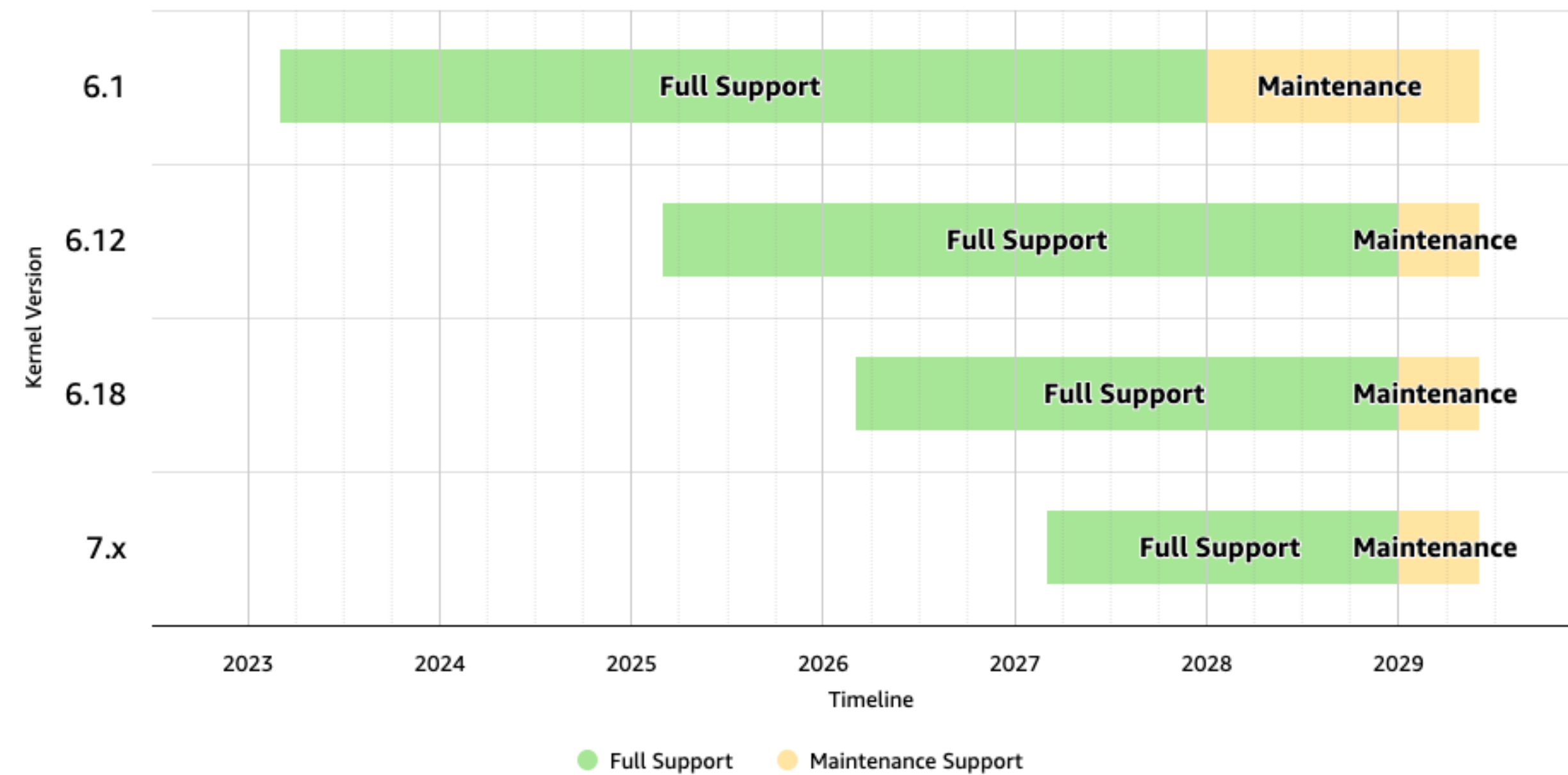
Amazon Linux 2023 Kernel Release Timeline
