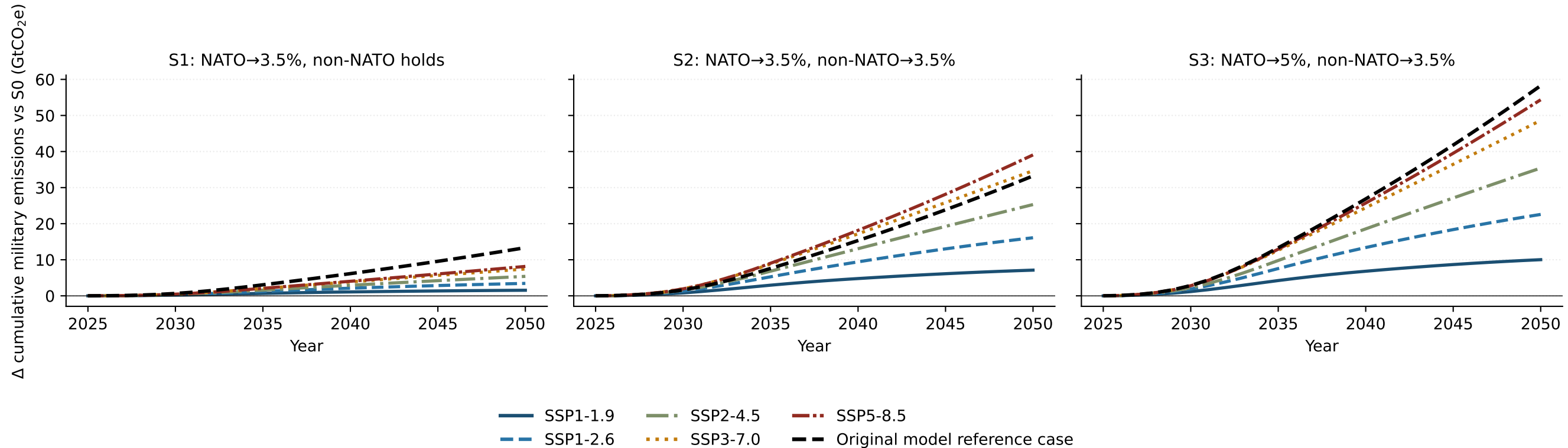
SA2: AR6 World GDP/GHG; dynamic SSP v3.2 NATO share Figure 4. Incremental cumulative military emissions relative to S0 (2025-2050)
