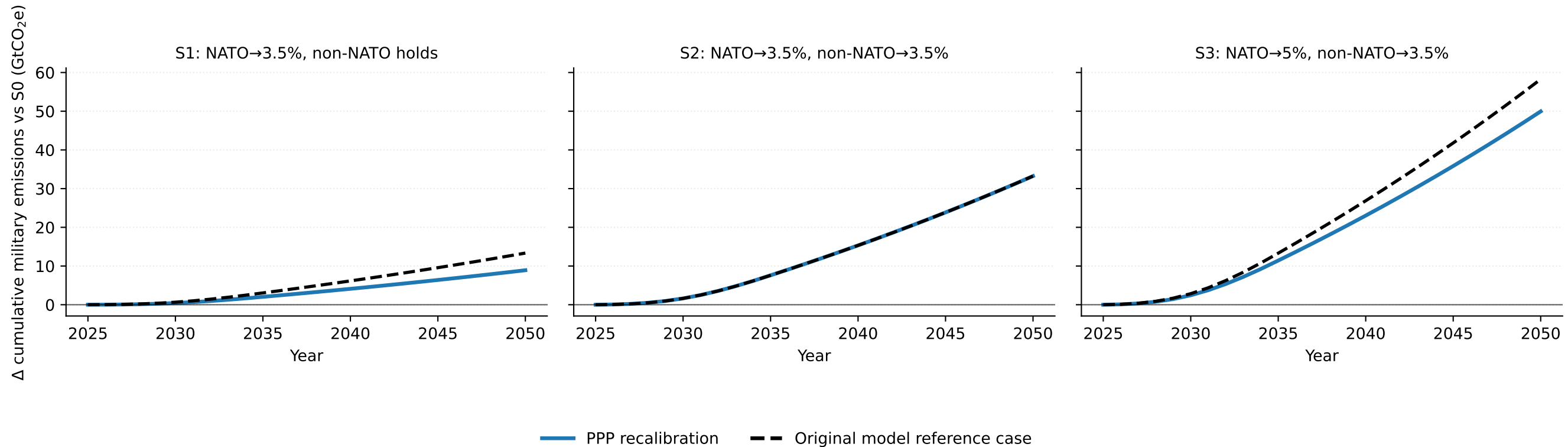
SA3: Original reference model recalibrated in PPP Figure 4. Incremental cumulative military emissions relative to S0
