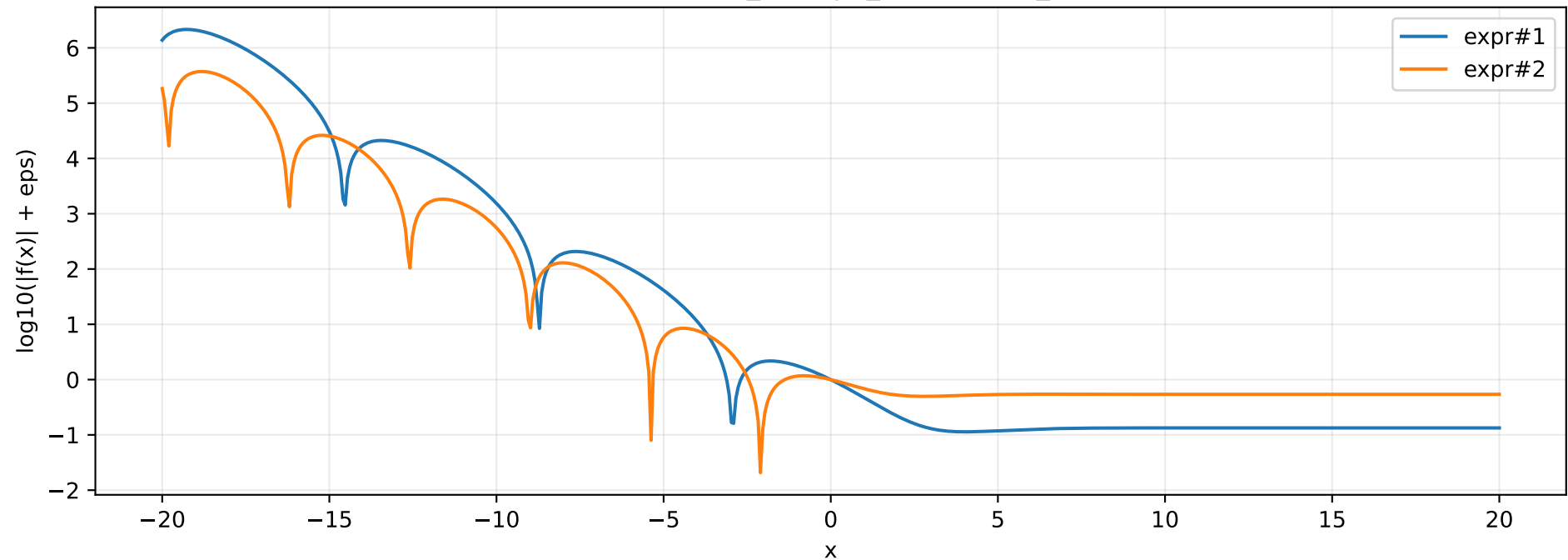
Fail examples: func_id=0 | n_fail=160 / n_all=1545
