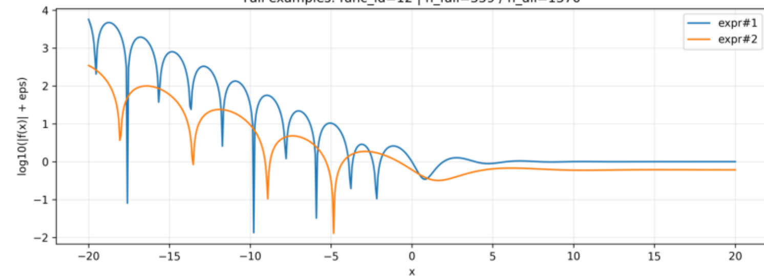
func_id=12 | Damped wave oscillation + damping / phase drift
