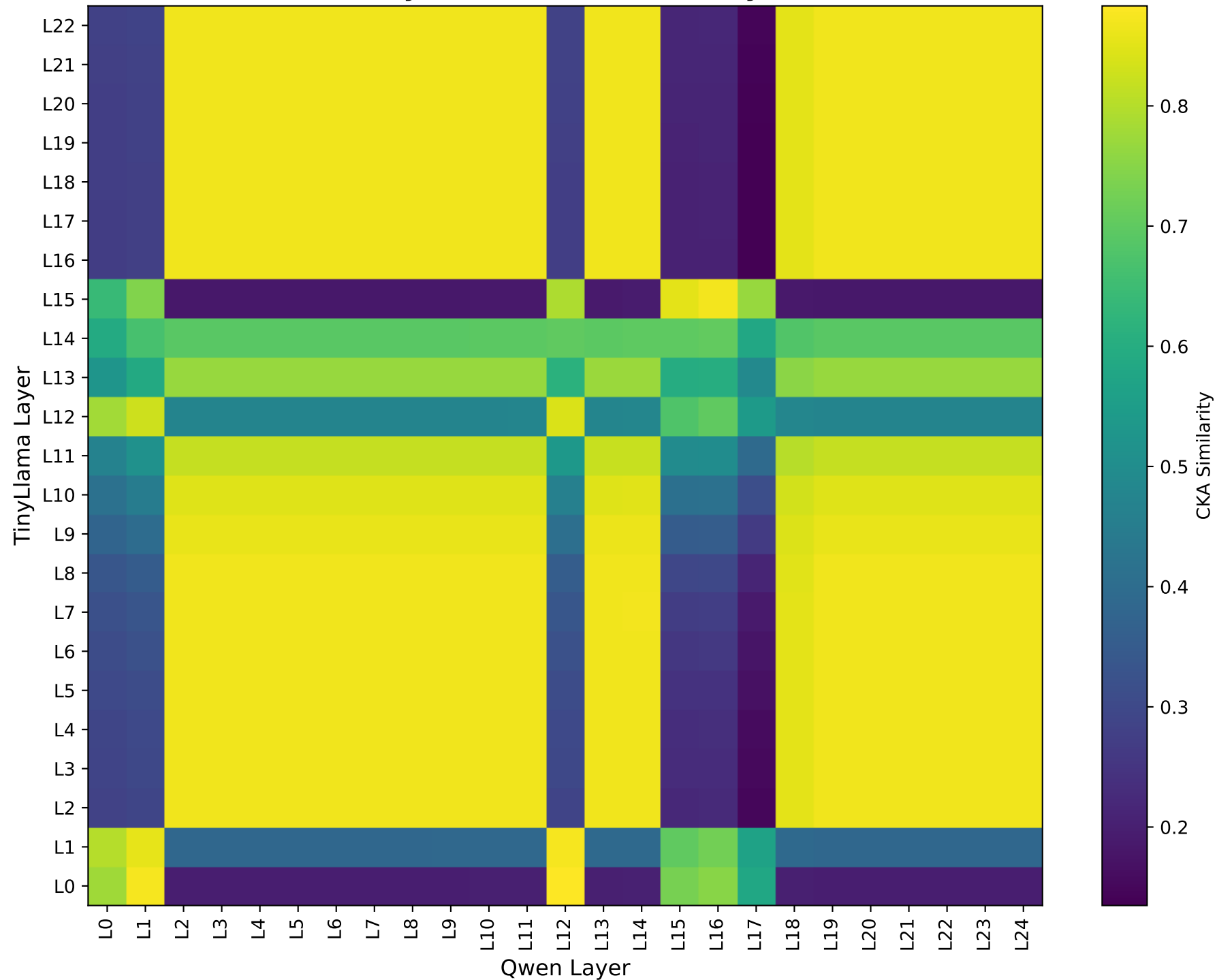
Layer-wise CKA Similarity
