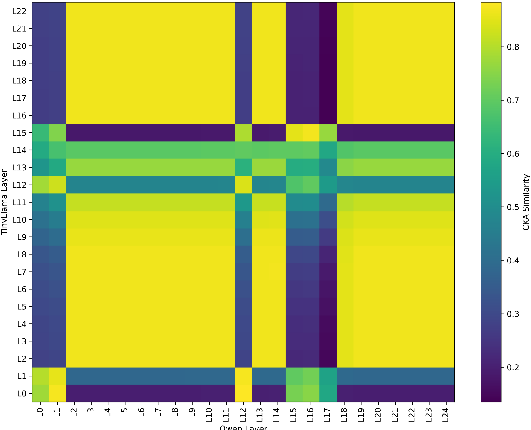
Layer-wise CKA Similarity
