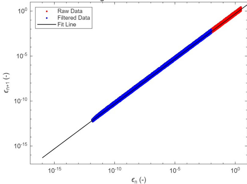
Error Convergence Plot for Bisection Root Solver
