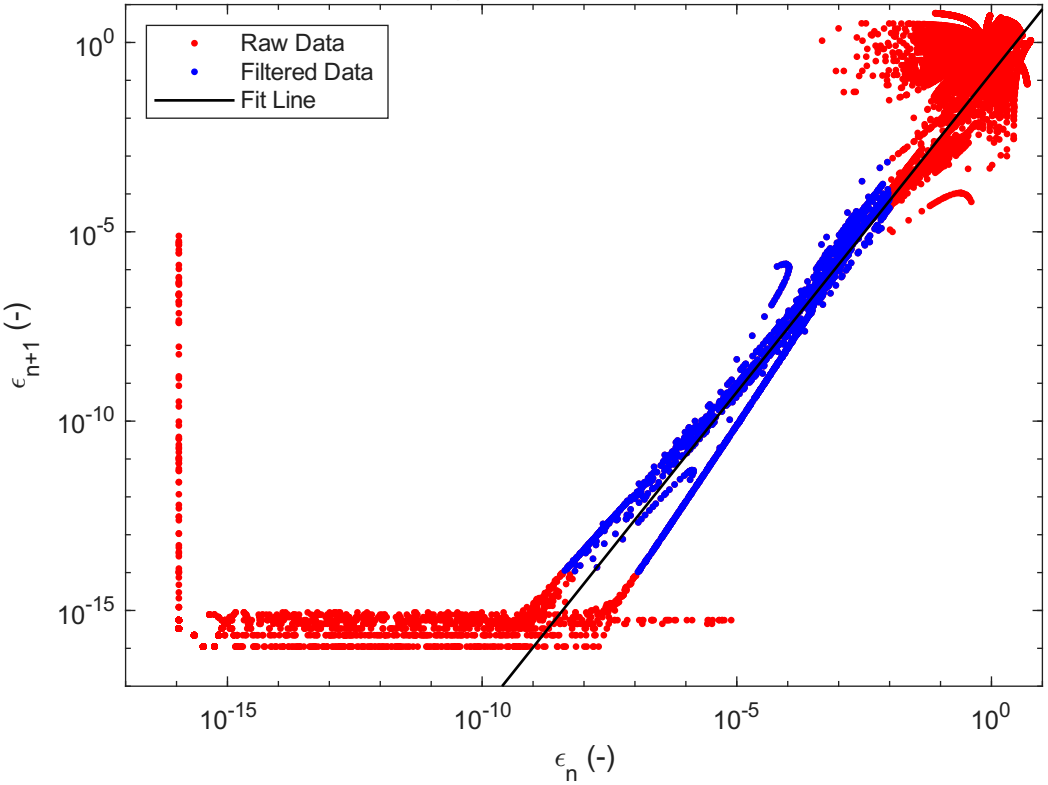
Error Convergence Plot for Fzero Root Solver
