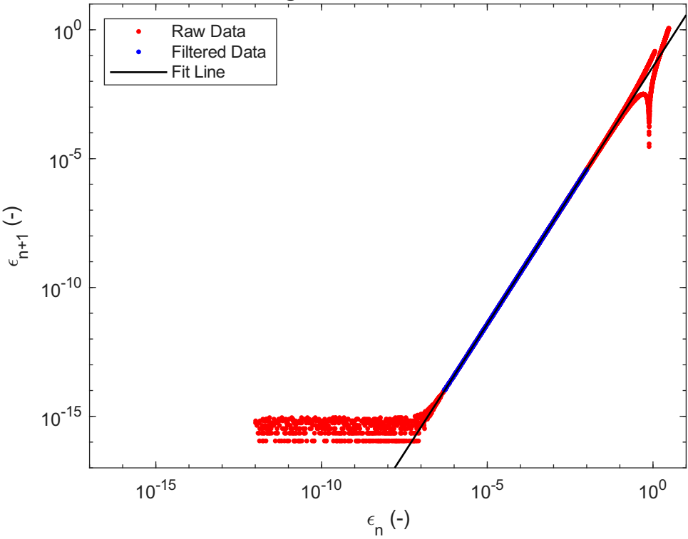
Error Convergence Plot for Newton Root Solver
