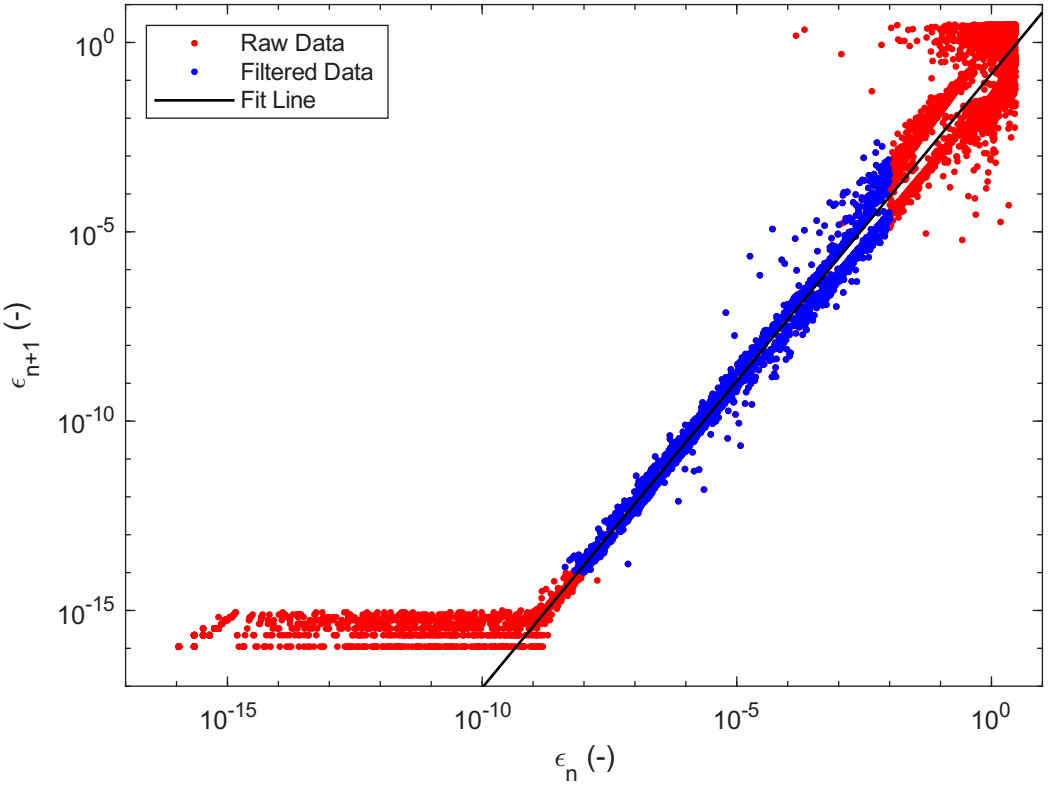
Error Convergence Plot for Secant Root Solver
