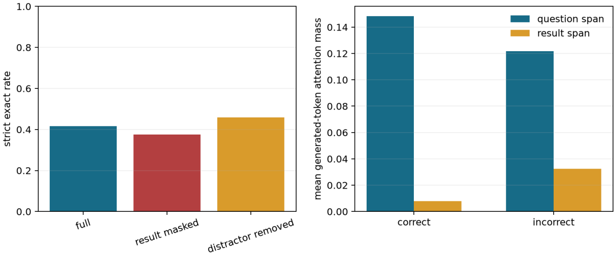
Figure 7: Left: strict causal-content ablations. Right: generated-token attention mass by outcome. Span lengths differ, so question-versus-result heights are not directly comparable; correct-versus-incorrect differences within a span are the relevant diagnostic.
