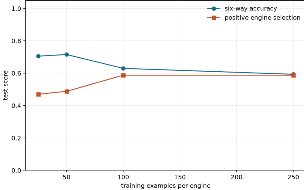
Figure 3: Word TF-IDF does not approach reliable six-way selection as the training set grows; increasing trigger recall is accompanied by control activation.
