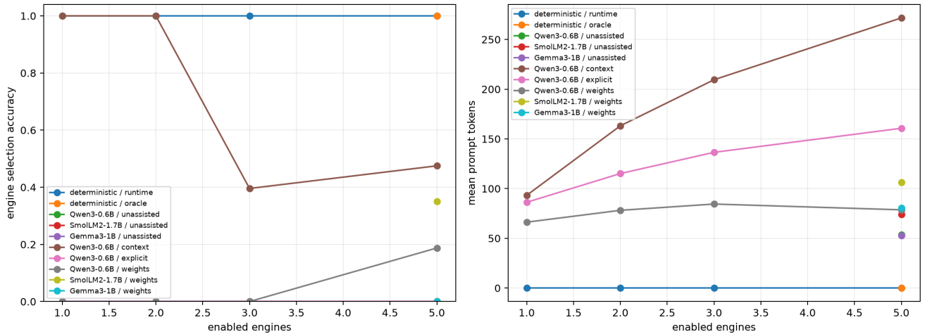
Figure 5: Engine selection and mean tokenizer prompt cost versus enabled engine count. Deterministic and oracle lines are protocol bounds, not learned evidence.
