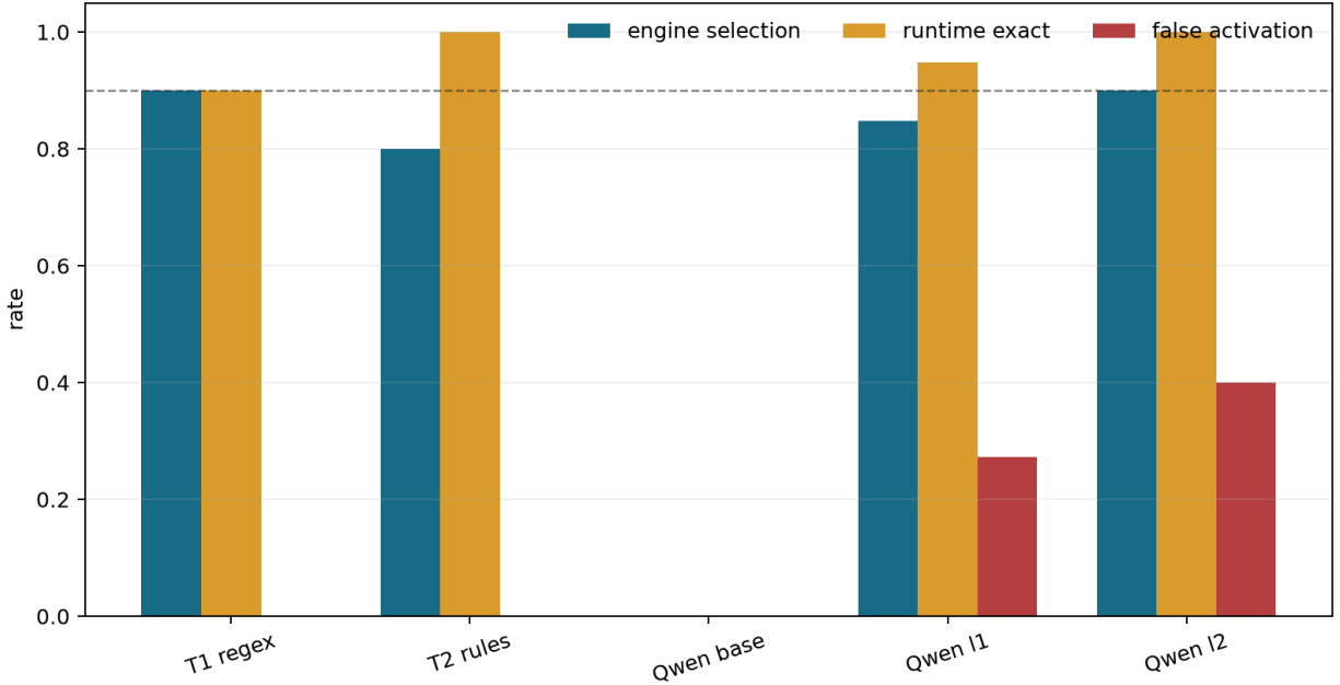
Figure 4: Factorized routing improves positive selection, but neither neural adapter meets the joint selection/runtime/FAR gate. The dashed line marks the 0.9 positive-rate threshold; FAR must independently remain at most 0.1.
