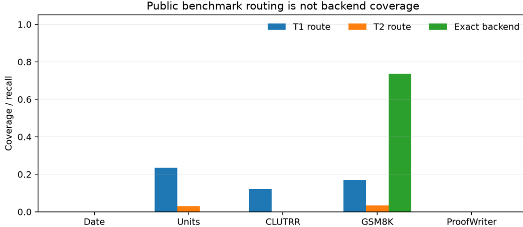
Figure 2: A correct assistance intent is not enough: transferred routing and exact-backend coverage remain distinct bottlenecks on public tasks.
