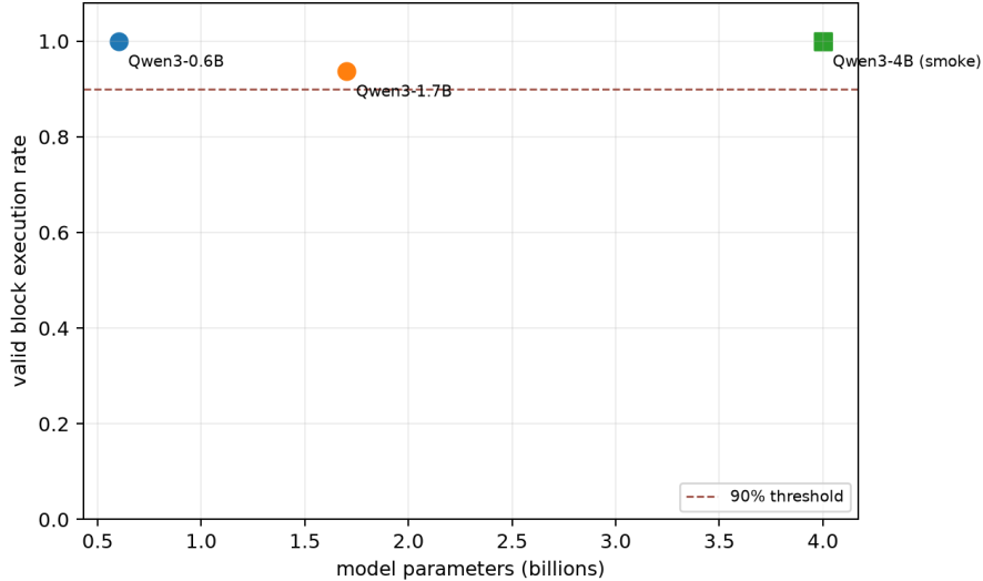
Figure 2: Valid execution under the one frozen ICL prompt. Circles are 16-example held-out diagnostics; the square is a four-example smoke and must not be read as a comparable estimate. Parameter count is descriptive, not a fitted scaling law.
