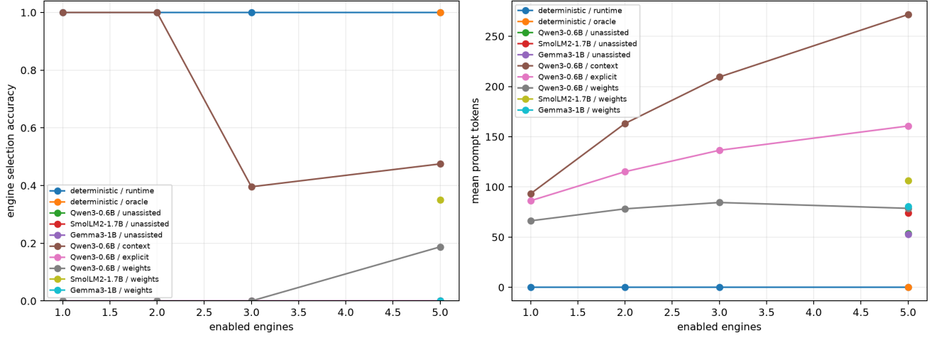
Figure 4: Engine selection and mean tokenizer prompt cost versus enabled engine count. Deterministic and oracle lines are protocol bounds, not learned evidence.
