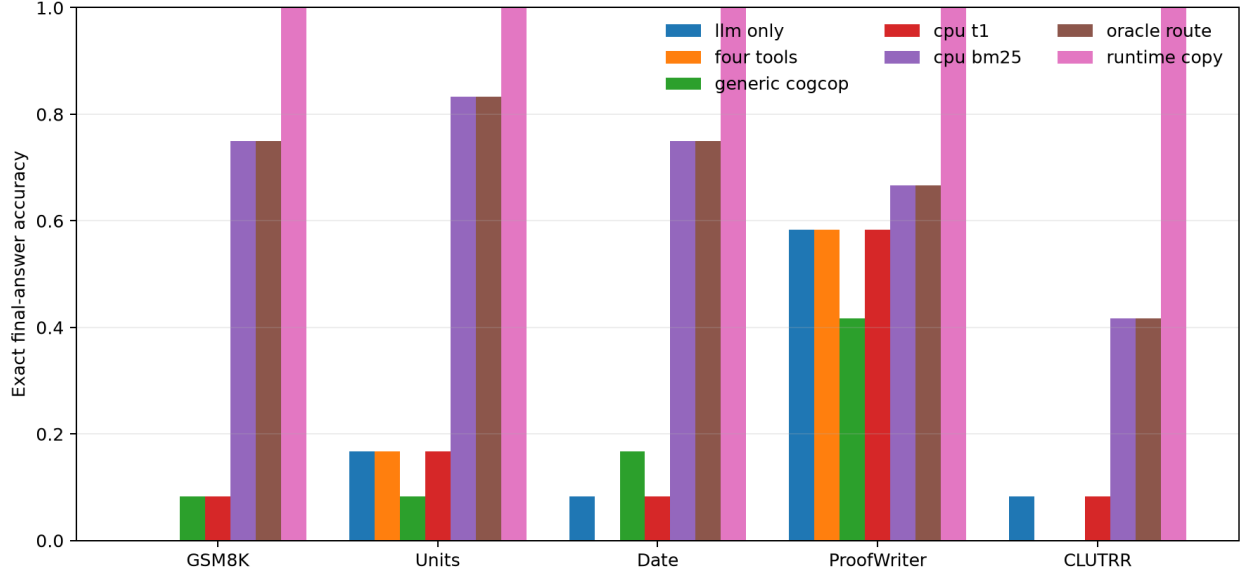
Figure 3: Matched public final accuracy. Perfect registered routing does not guarantee that Qwen preserves an exact result; direct runtime-copy does.
