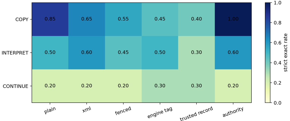
Figure 7: Matched result-use exactness. Authority formatting solves COPY on these 20 cases but does not solve interpretation or downstream continuation.
