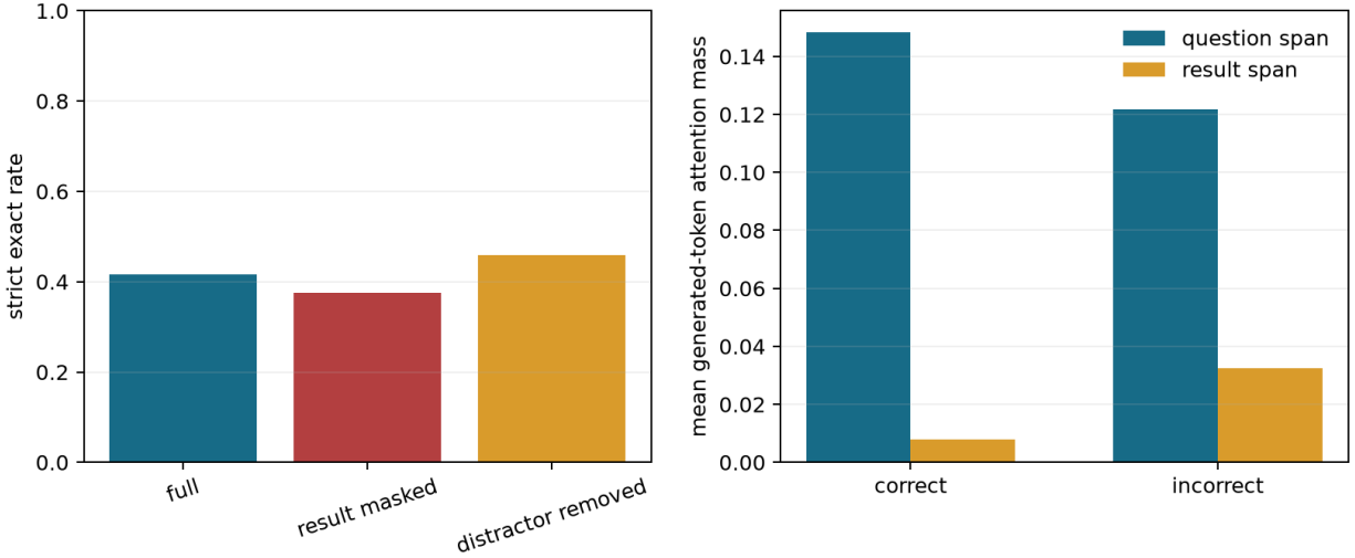
Figure 8: Left: strict causal-content ablations. Right: generated-token attention mass by outcome. Span lengths differ, so question-versus-result heights are not directly comparable; correct-versus-incorrect differences within a span are the relevant diagnostic.
