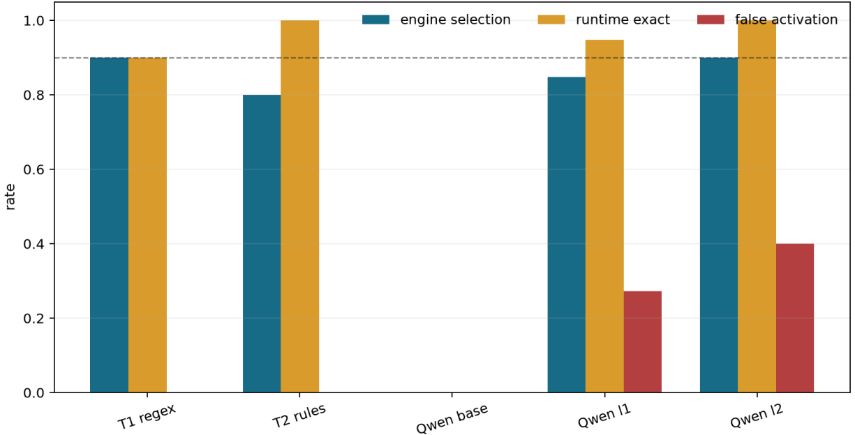
Figure 5: Factorized routing improves positive selection, but neither neural adapter meets the joint selection/runtime/FAR gate. The dashed line marks the 0.9 positive-rate threshold; FAR must independently remain at most 0.1.
