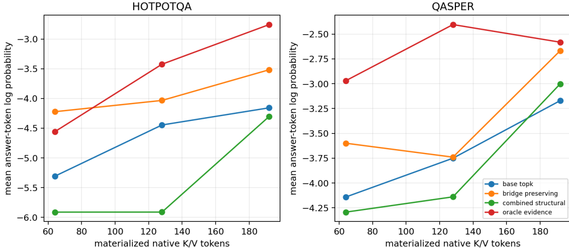
Figure 3: Natural frozen-Qwen quality versus measured native K/V tokens. Bridge means exceed B0 throughout, but paired uncertainty includes zero; S5 fails to generalize reliably.
