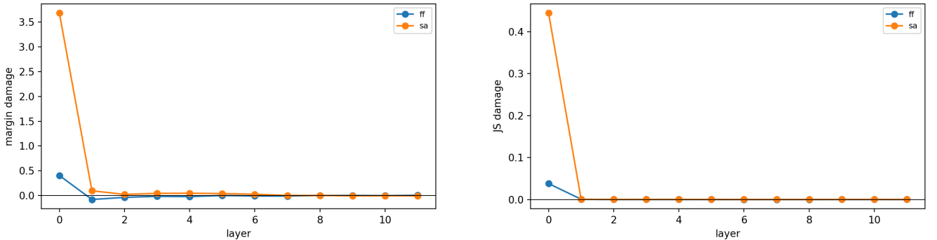
Figure 7: Cross-tree role replacement (left) and component intervention (right), restricted to competent local cells. SA is substantially more causally sensitive than FF.
