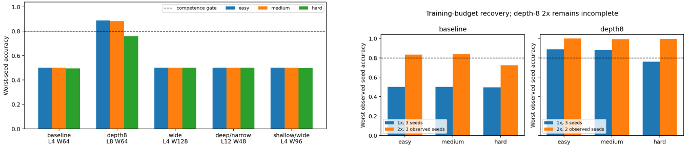
Figure 5: Left: worst-seed isAncestor accuracy for selected one-budget allocations. Right: observed training-budget comparison. Baseline 2x contains all three seeds; depth-eight 2x contains only seeds 11 and 23 and is not a central gate.
