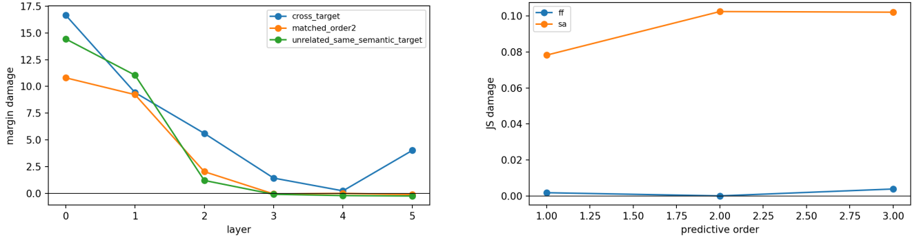
Figure 8: S3 causal completion. Role-matched order-2 donors are less damaging than cross-target controls (left); SA/FF sensitivity changes with predictive order (right).
