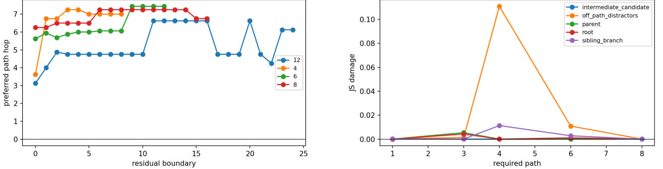
Figure 6: Locally competent isAncestor cells only. Preferred decoded path position (left) lacks a seed-stable iterative trajectory; intermediate masking is nearly harmless compared with endpoint masking (right).
