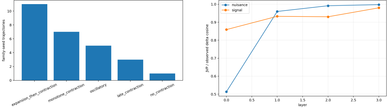
Figure 8: Trajectory classes and local JVP agreement. Median JVP/observed cosine is 0.984 for nuisance and 0.928 for signal directions; prediction-space relative errors are 0.179 and 0.311.
