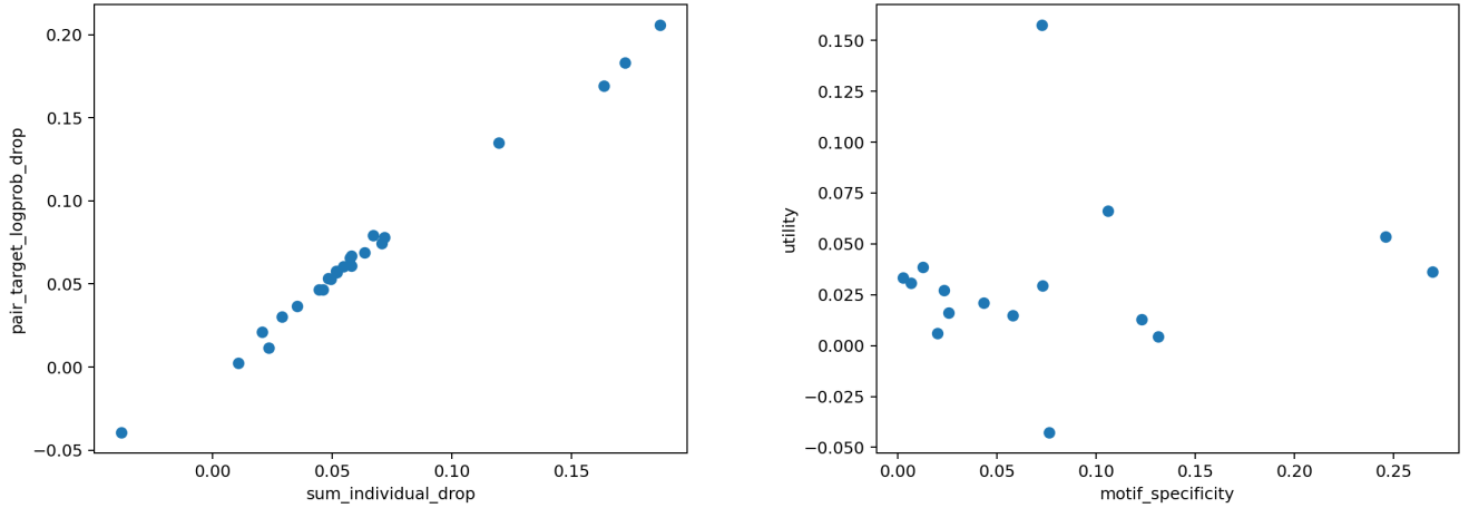
Figure 15: Non-additive pair effects and the repeated motif-causal null.
