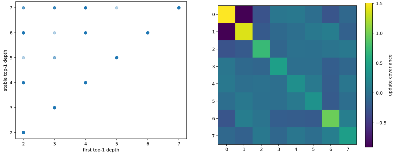
Figure 7: First versus stable decision boundaries and cross-boundary margin-update covariance. Negative off-diagonal structure implements fluctuation cancellation/repair.
