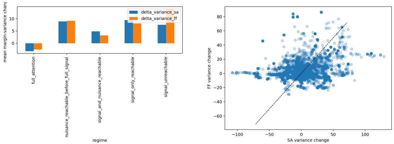
Figure 13: Mean sublayer variance changes by reachability regime and cellwise SA versus FF changes. SA is important, but not uniquely dominant, and the sign depends on learned competence.
