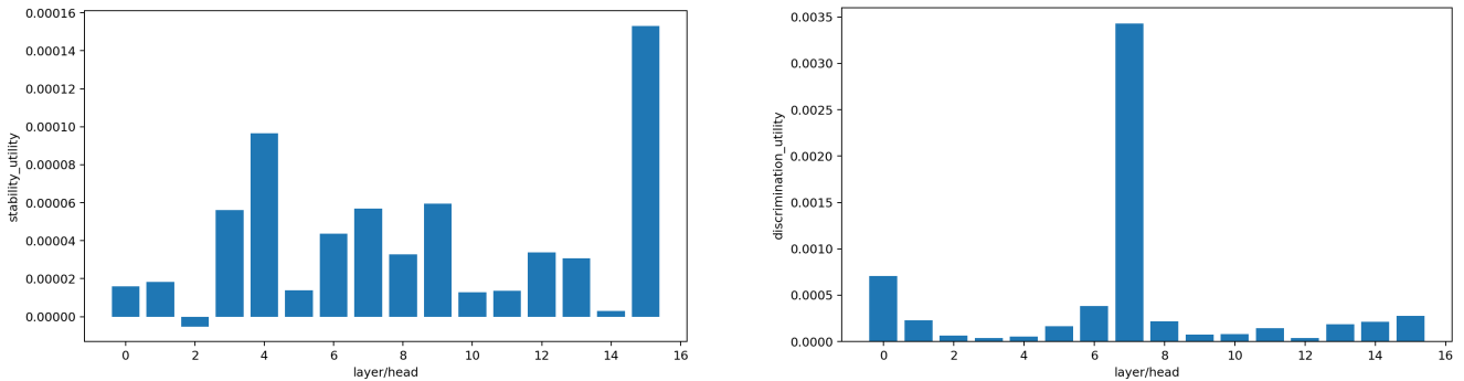
Figure 14: Causal stability and discrimination utilities for all layer/head cells.
