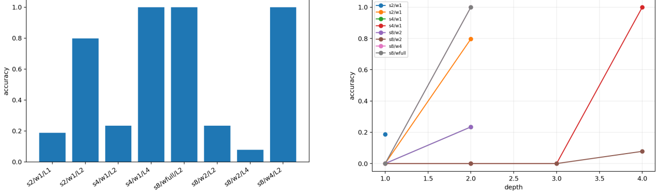
Figure 10: Final accuracy by span/window/depth cell and layerwise functional arrival.
