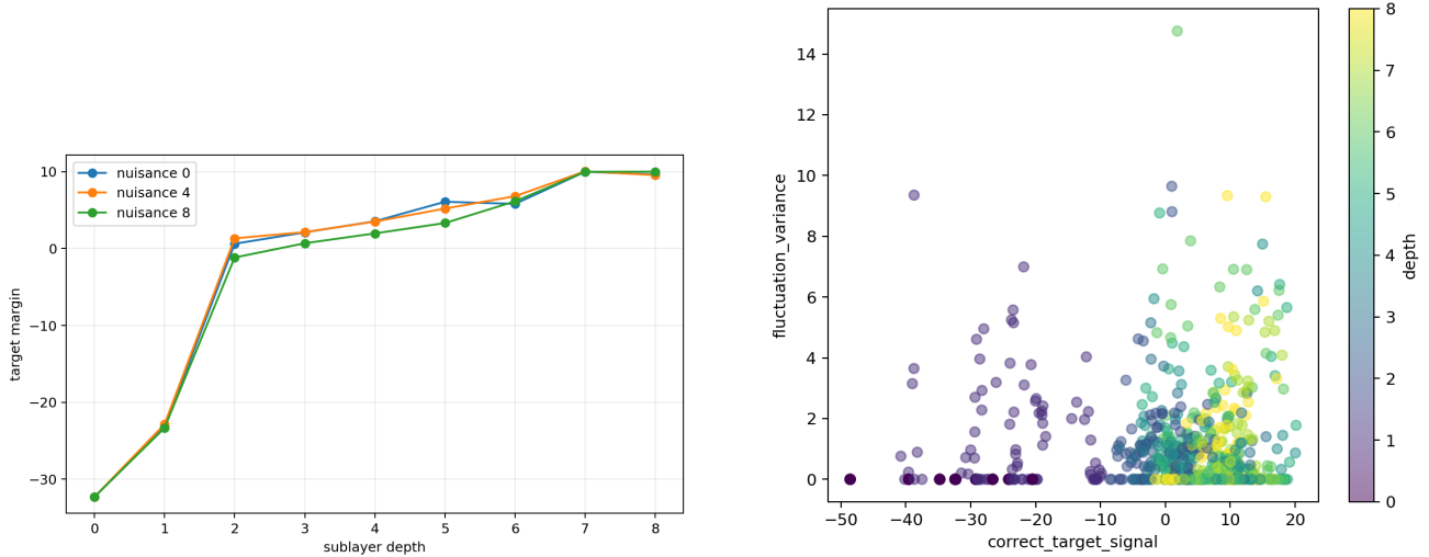
Figure 6: Correct-target margin across sublayer depth and the signal–fluctuation phase plane. The trajectory moves from confidently wrong and identical to confidently correct with finite nuisance variation.
