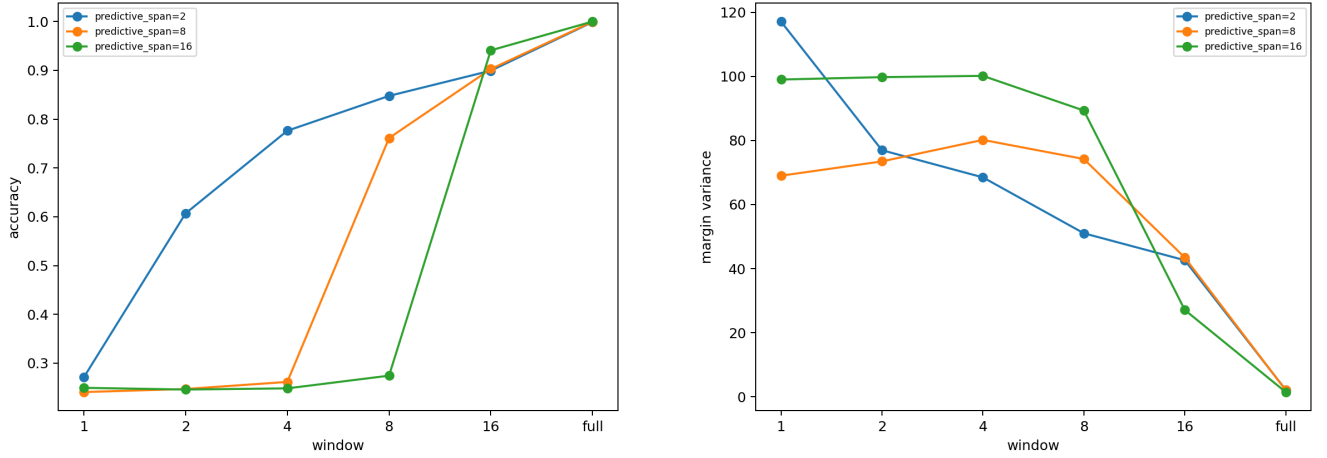
Figure 11: Full-trained models under inference-time window restriction. Accuracy and margin variance improve toward full exposure; reachability alone does not preserve the learned computation.
