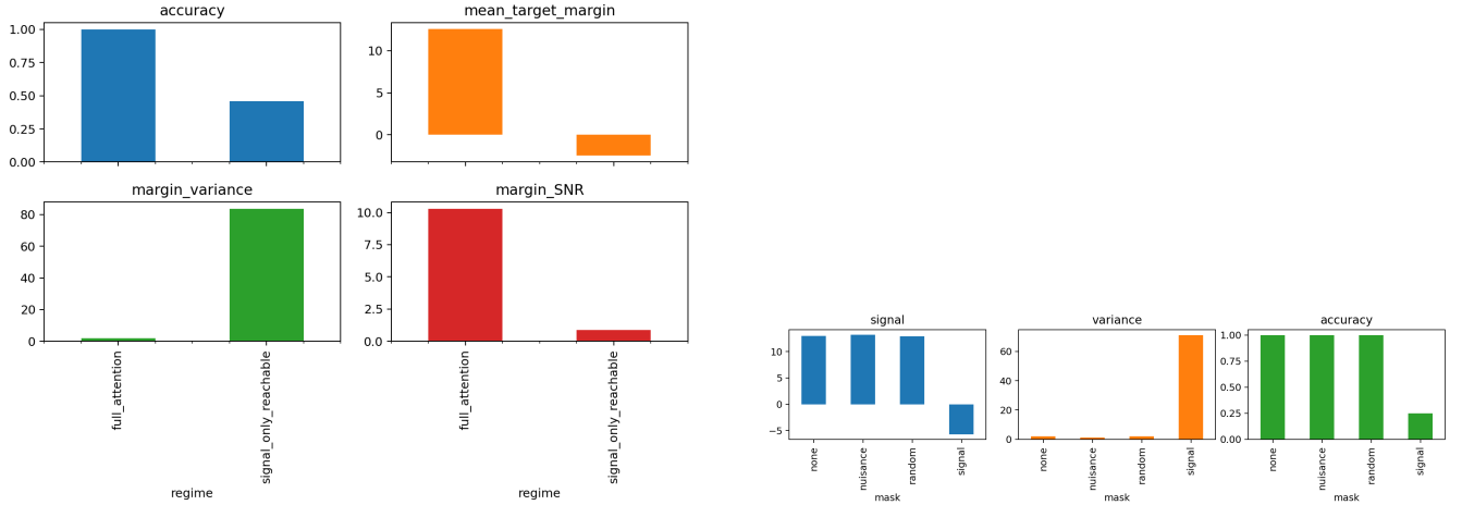
Figure 12: Left: graph-defined signal-only reachability does not match full-attention competence without local-window training. Right: selective nuisance removal lowers variance without sacrificing signal, while signal removal collapses performance.
