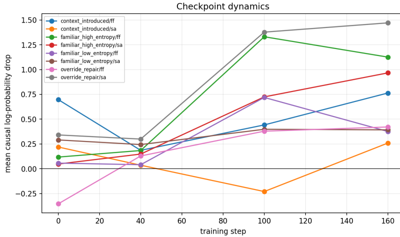
Figure 7: Component causal contribution over local training checkpoints. The trajectories are retained even when they do not match a monotone compilation account.
