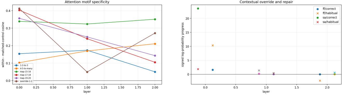
Figure 6: Left: motif specificity by relation and layer. Right: signed progress for habitual and contextually correct continuations. Geometry labels in the raw artifact remain candidates until paired with task-conditioned causal and temporal evidence.
