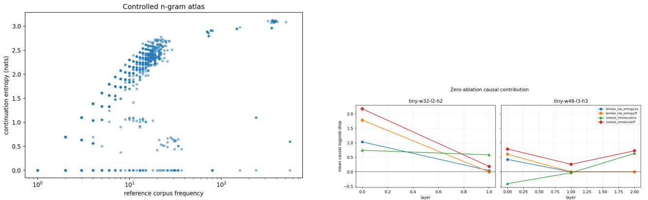
Figure 1: Left: controlled atlas frequency–entropy support. Right: layerwise zero-ablation effects for the two model settings. Curves include all pre-registered strata; the displayed comparison emphasizes familiar low-entropy and context-introduced mappings.
