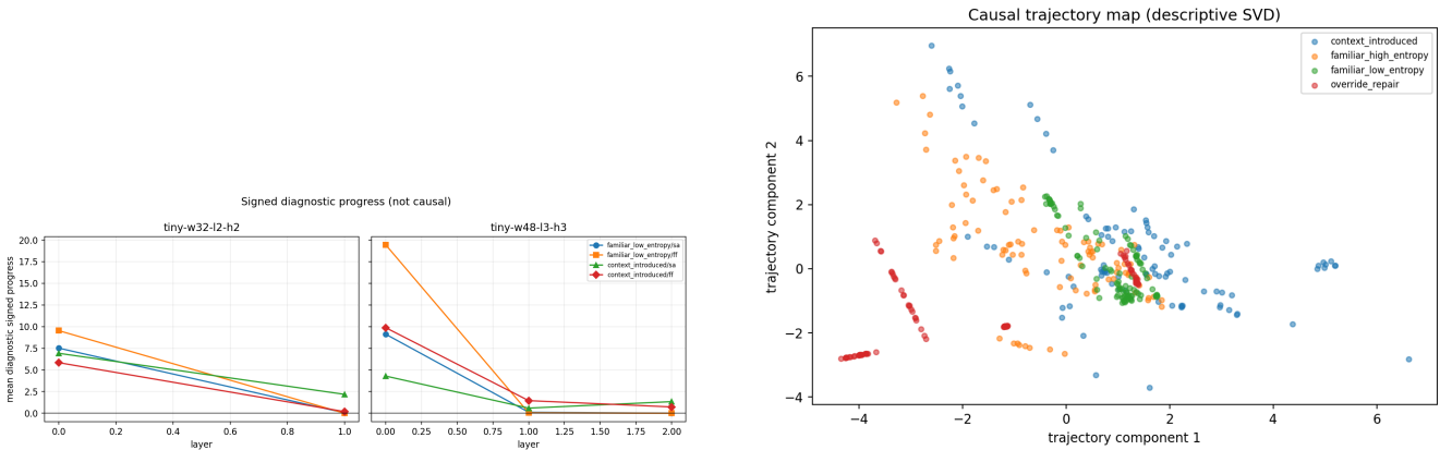
Figure 5: Left: signed diagnostic progress, explicitly not a causal effect. Right: descriptive SVD of per-example causal trajectories; cluster appearance is exploratory and no discrete mechanism classes are asserted.
