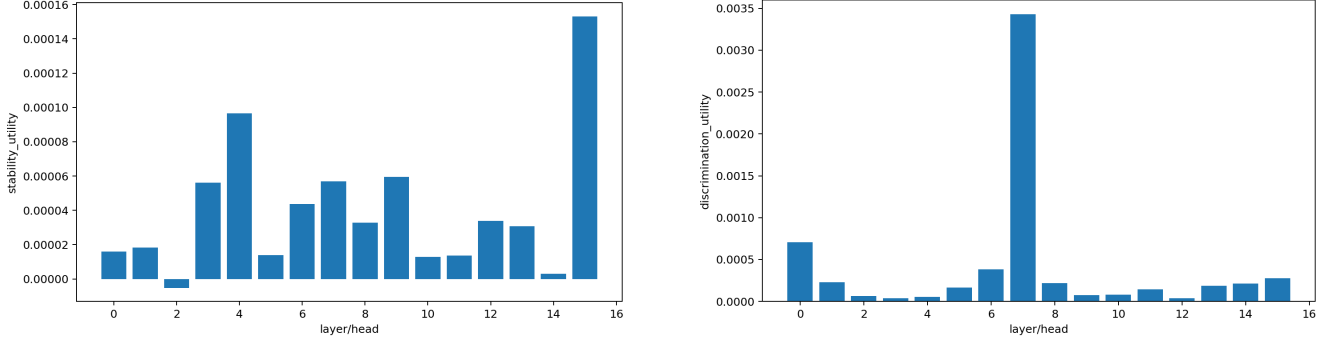
Figure 9: Causal stability and discrimination utilities for all layer/head cells.
