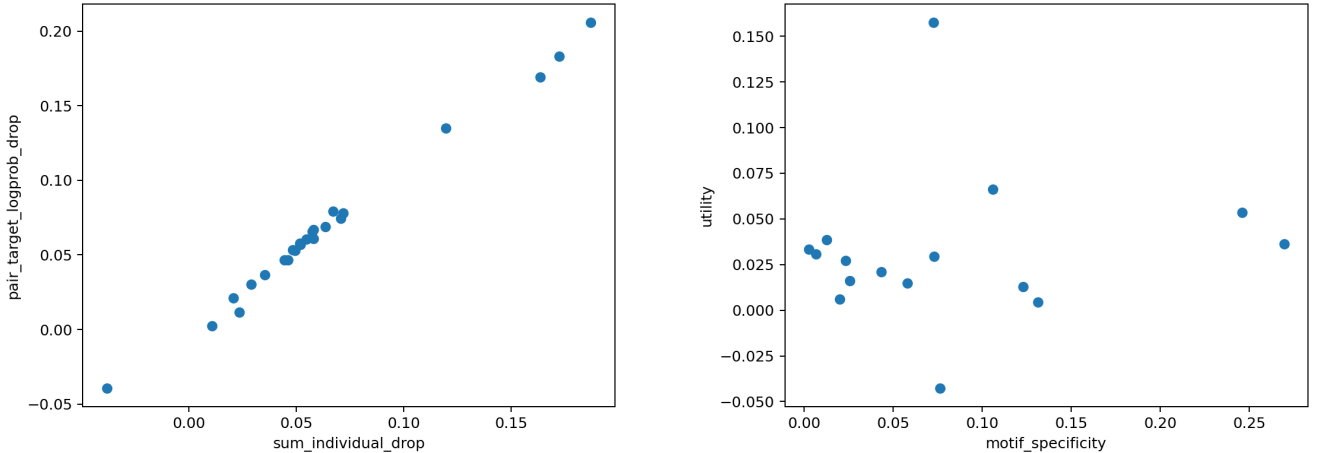
Figure 10: Non-additive pair effects and the repeated motif-causal null.
