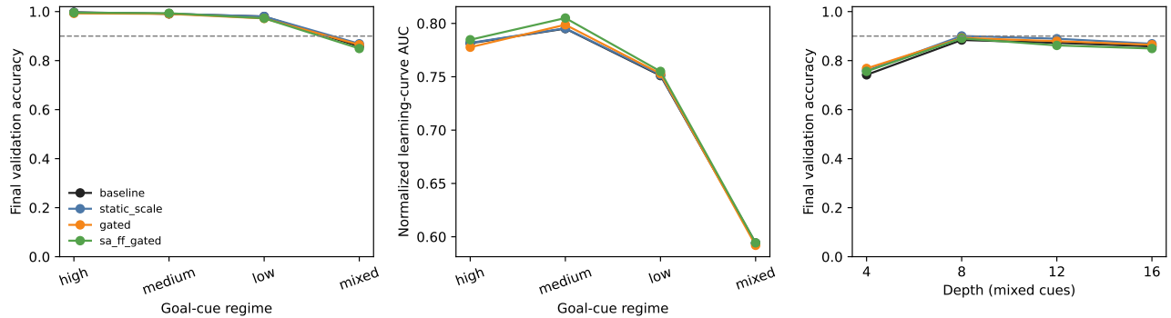
Figure 9: C2 goal-cue and mixed-depth results. Dashed lines mark the .90 validation threshold. Mixed-cue performance is non-monotonic in depth and highly seed-sensitive.
