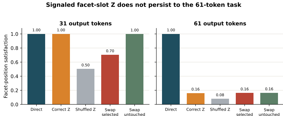
Figure 2: One-seed horizon diagnostic. Direct text remains perfect at 61 tokens, while correct-Z generation and slot-swap locality collapse relative to 31 tokens. Shuffled Z is shown to distinguish residual example-specific use from schedule-prior behavior.
