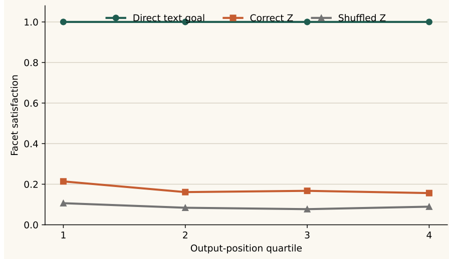
Figure 4: Facet satisfaction after the extended matched budget. Direct goal access reaches ceiling in every output quartile; correct Z_G remains low but above shuffled Z_G . Source: results/horizon_32_extended_optimization_iteration1.csv .
