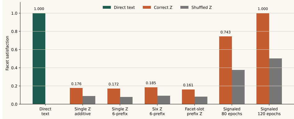
Figure 3: Matched 31-token conditioning comparison. Explicit identity and position signals sharply improve facet-slot Z; with extended optimization it reaches the direct-text ceiling while preserving a large correct-versus-shuffled gap. Source: results/horizon_32_conditioning_comparison_iteration1.csv.
