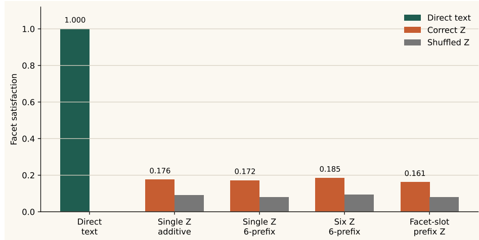
Figure 2: Matched 31-token conditioning comparison. Neither continuous-prefix presentation, generic six-vector encoding, nor explicit facet slots close the large gap to direct text, while correct Z remains only modestly above shuffled Z. Source: results/horizon_32_conditioning_comparison_iteration1.csv .
