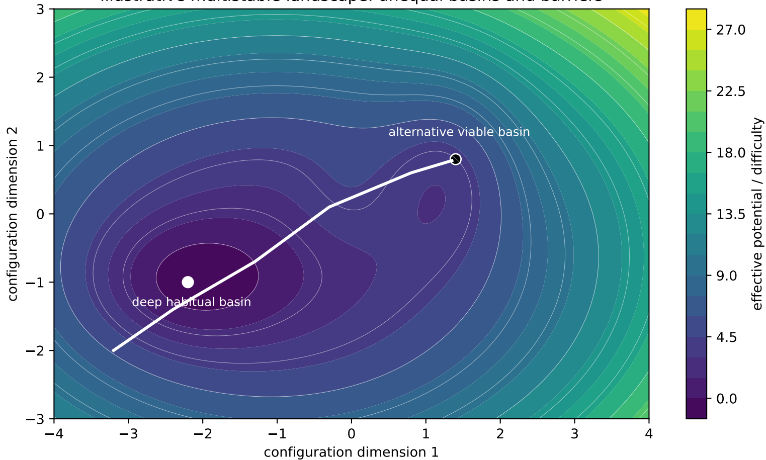
Illustrative multistable landscape: unequal basins and barriers
