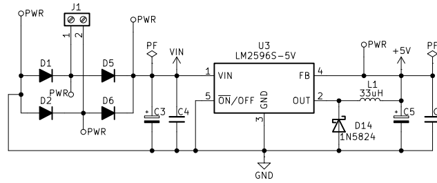
POWER SUPPLY
