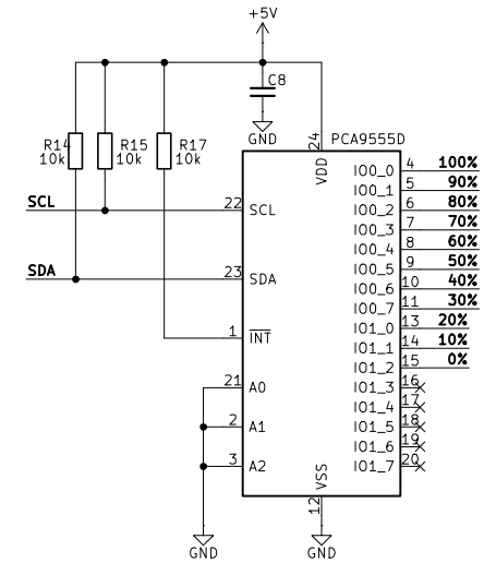
GPIO EXPANDER
