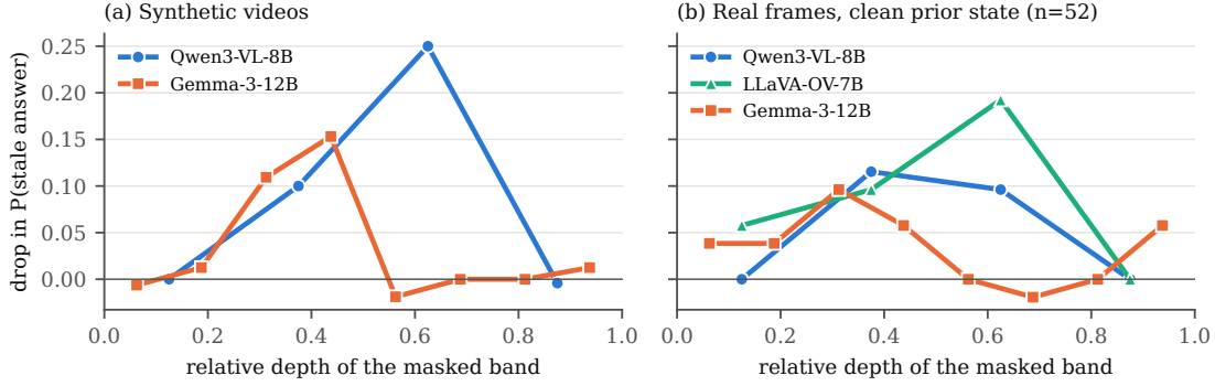
Figure 3. The stale answer is retrieved in middle layers. Drop in P(\text{stale}) when the question tokens are blocked from the previous state’s visual tokens within one band of layers (x: band center divided by the number of layers). (a) Synthetic videos: Qwen3-VL-8B ( n = 240 , D_{\text{fin}} \leq 1 s) and Gemma-3-12B ( n = 320 ). (b) Real frames with a clean prior state held 4 s (§7; n = 52 per model). Shallow and deep bands have no effect.
