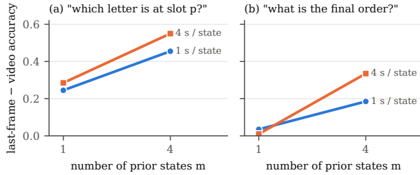
Figure 2. More prior states, and longer ones, make the present staler. Pooled last-frame minus video accuracy (5 models, n = 67 each; averaged over 2 and 4 fps, which had no effect). The final state is held 0.5 s. (a) Position questions. (b) Order questions, which need all letters: with a single prior state they show no gap.
