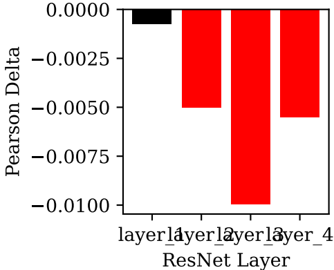
Pearson Delta vs. ResNet Layer
