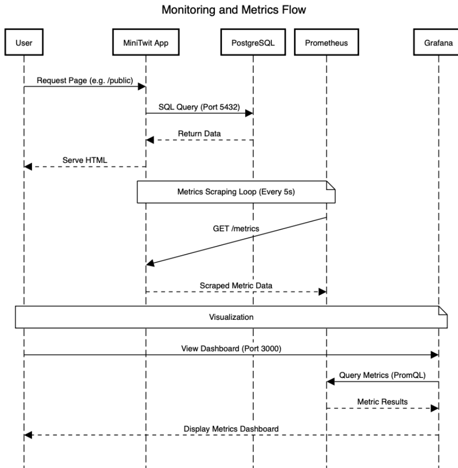
Figure 5: UML Sequence Diagram showing Monitoring flow
