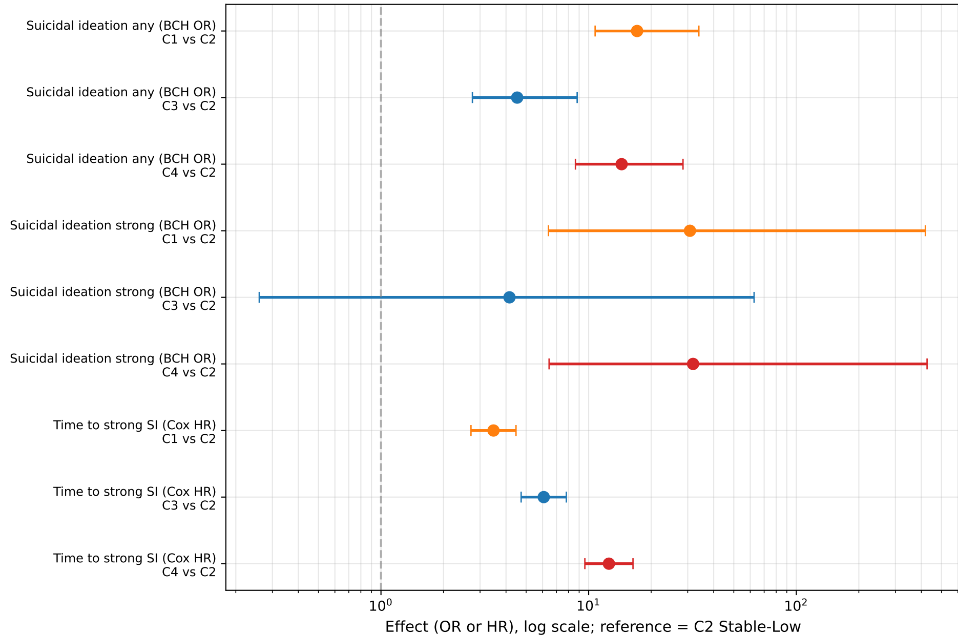
Figure 4. BCH-corrected distal outcome ORs and Cox HRs by trajectory class
