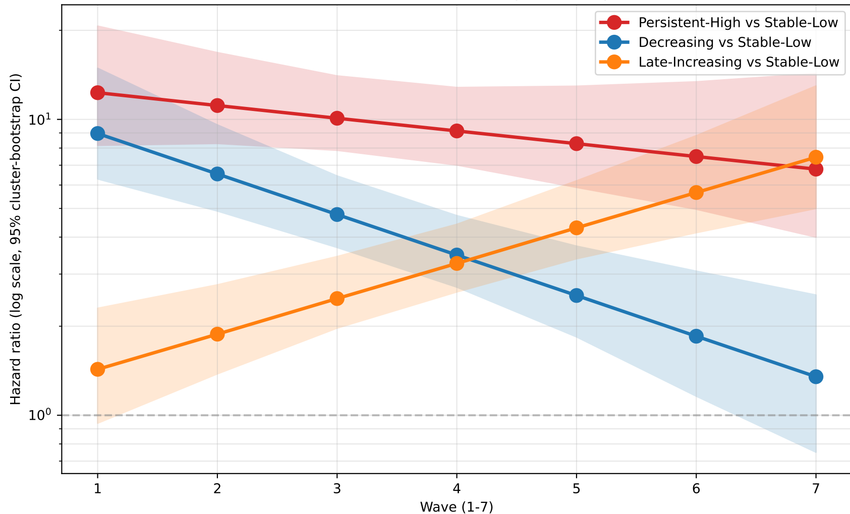
Figure 6 (BOOTSTRAP). Time-varying class HR for first strong SI Cox class \times wave; ID-level cluster bootstrap (B=300) percentile 95% CI
