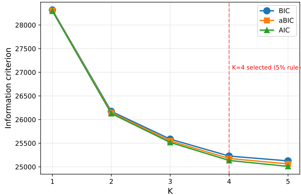
A. Information criteria (9-item primary)
