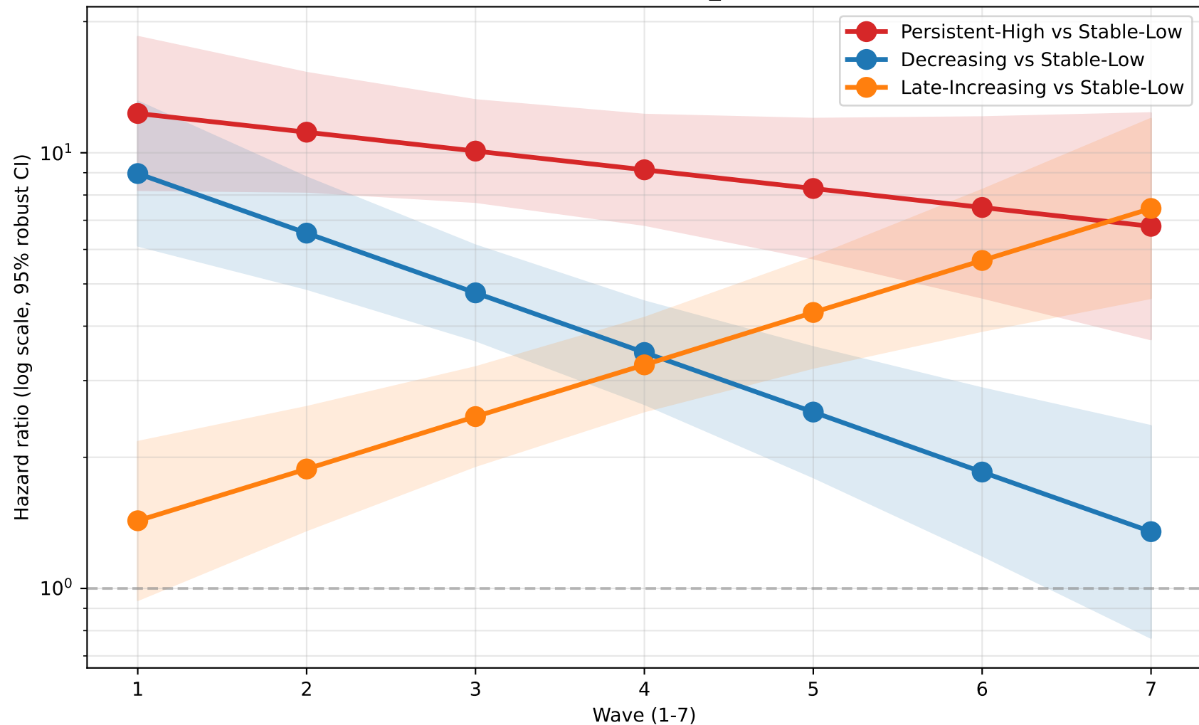
Figure 6 (REVISED). Time-varying class HR for first strong SI Cox class \times wave with cluster_col=ID, robust SE
