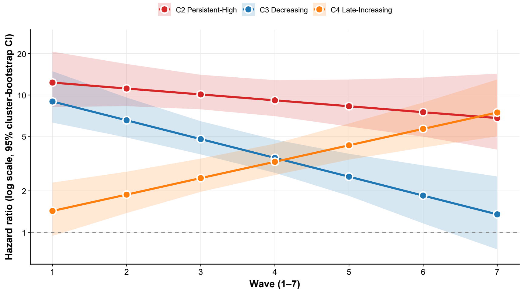
Figure 6. Time-varying class hazard ratios for first strong SI
