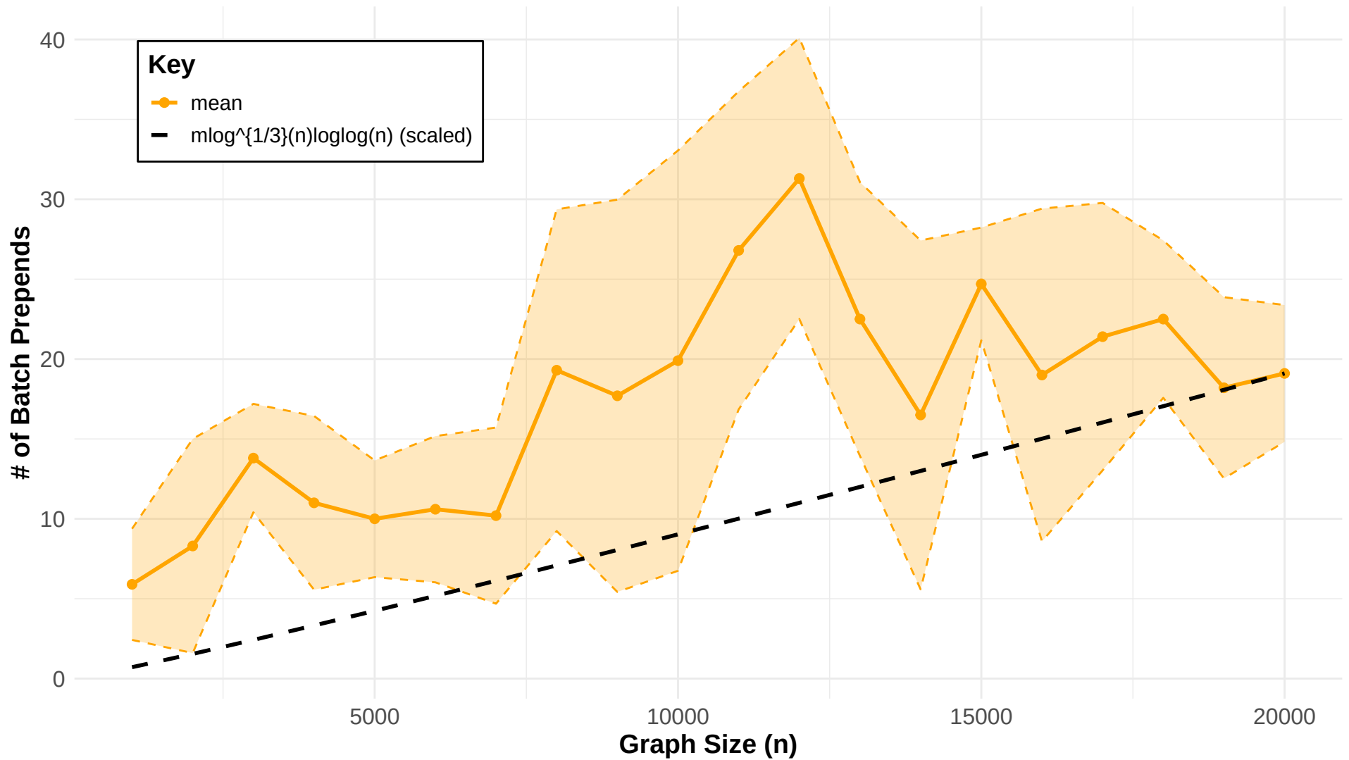
BMSSP Batch Prepends (mean \pm 1 sd)
