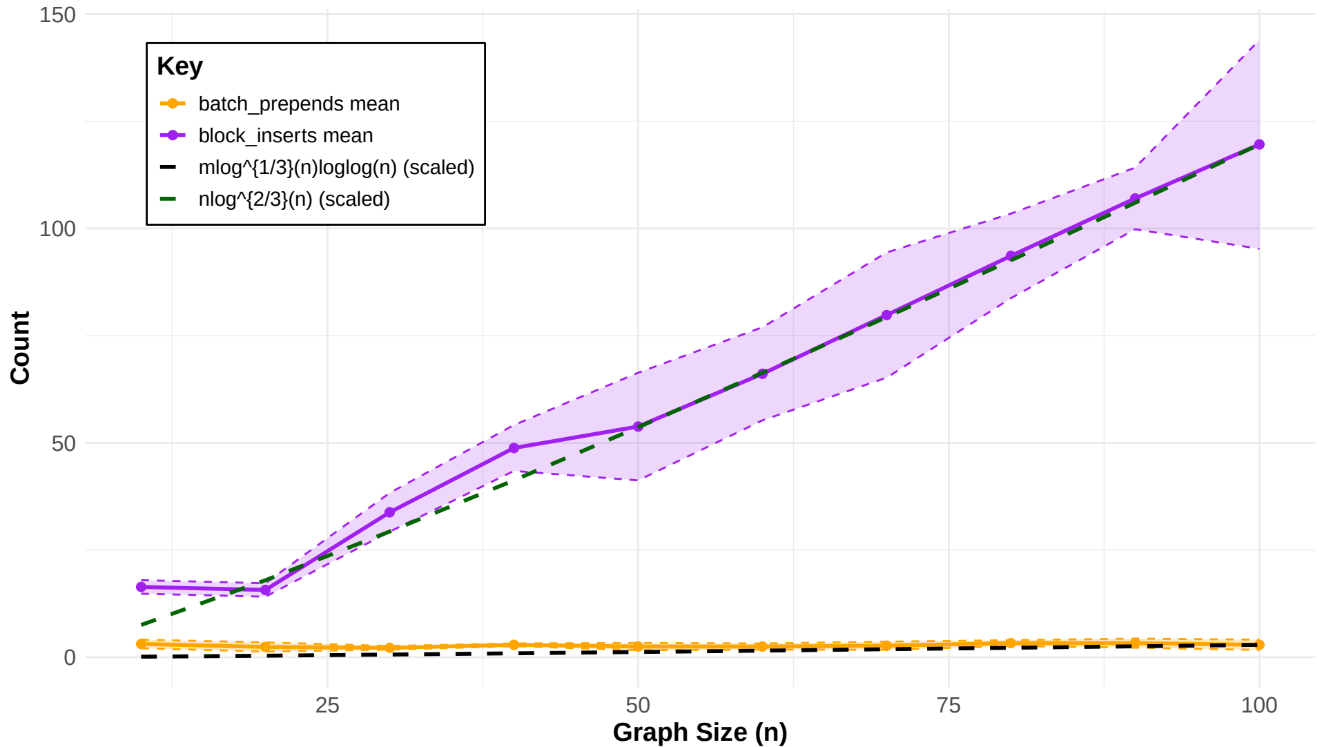
BMSSP Batch Prepends + Block Inserts (mean \pm 1 sd)
