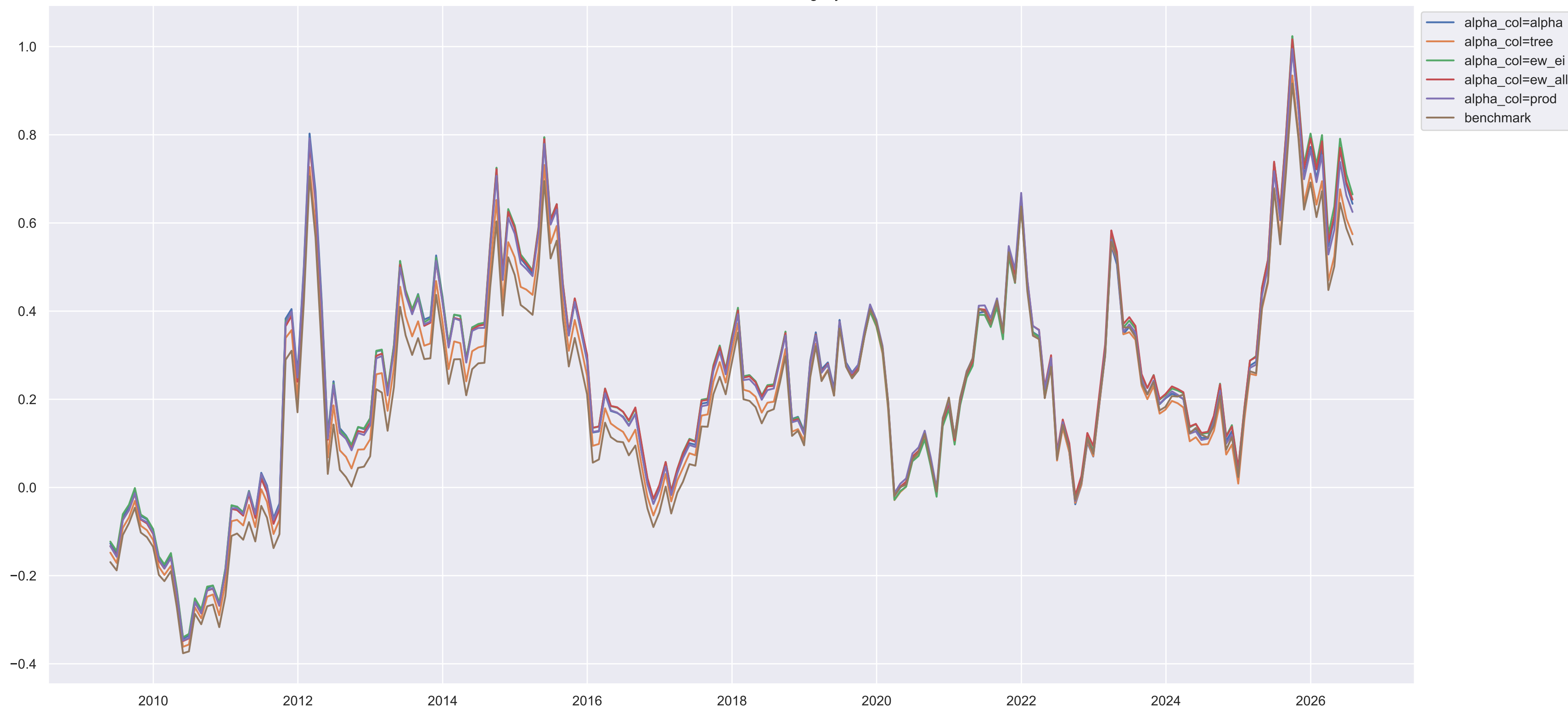
EU Absolute Performance Rolling 3 year
