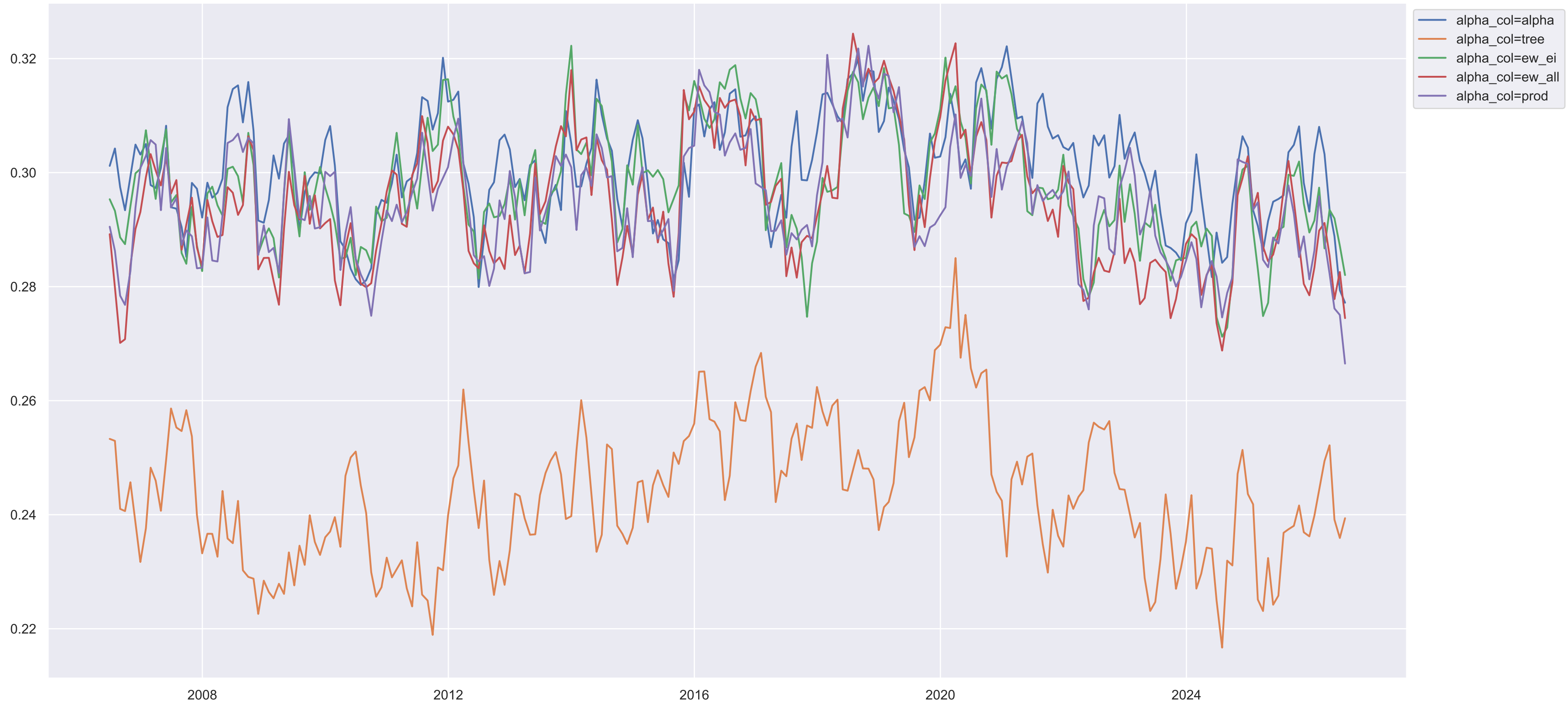
EU Active Share
