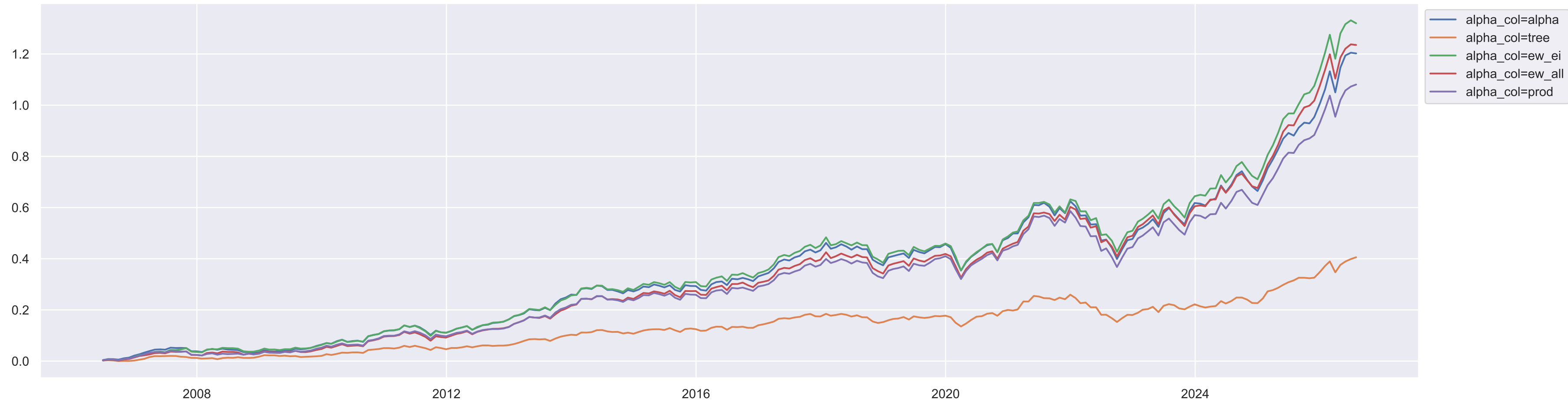
EU Active Performance
