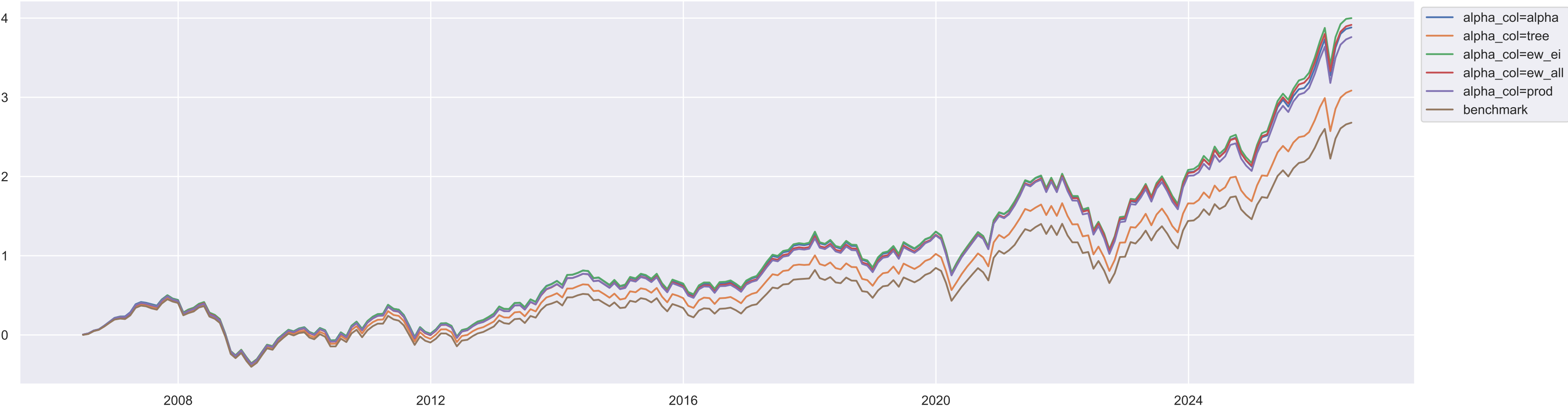
EU Absolute Performance
