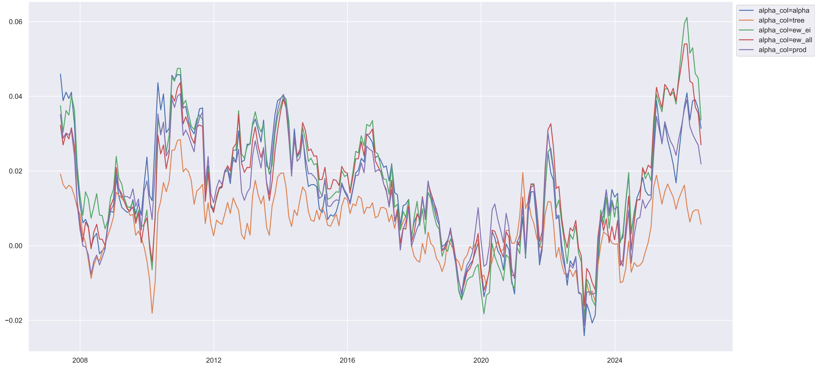
EU Active Performance Rolling 1 year
