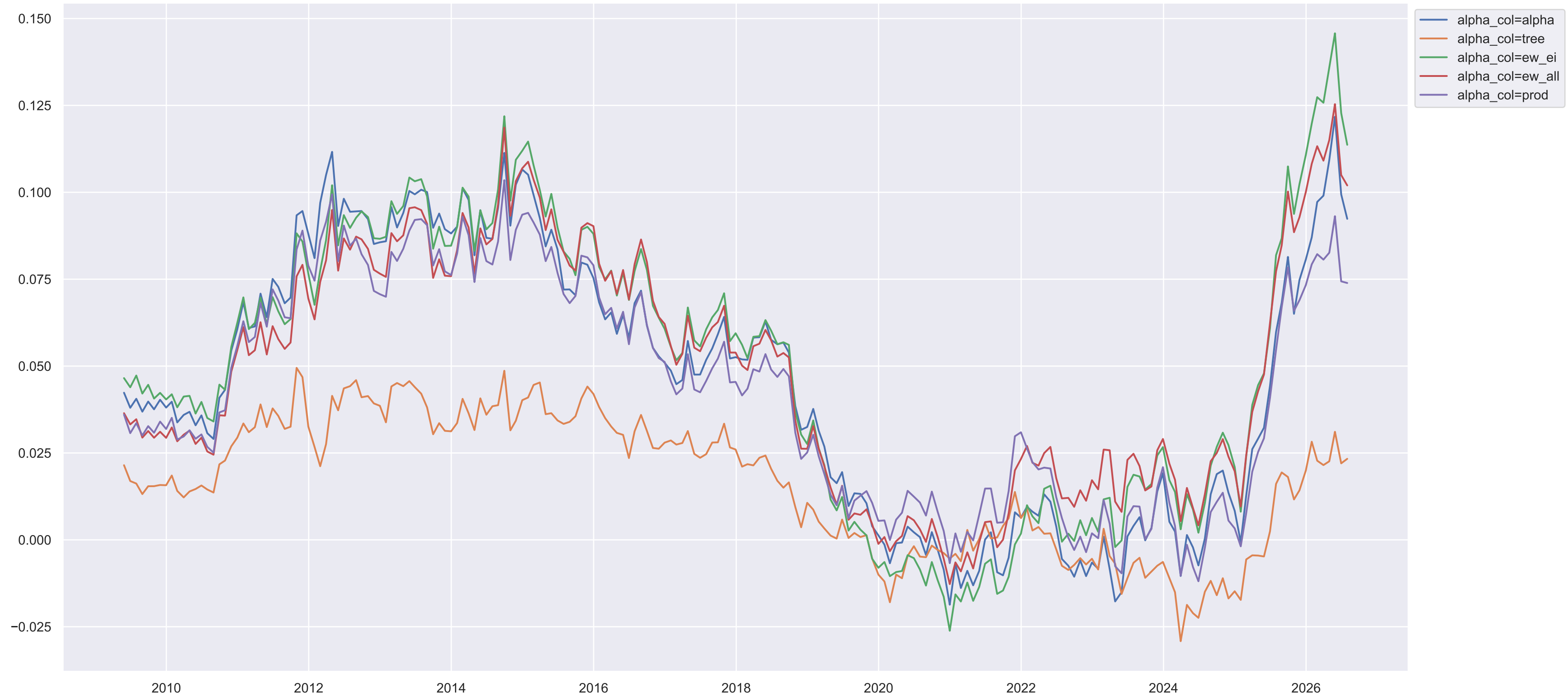
EU Active Performance Rolling 3 year
