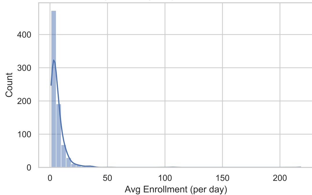
Histogram of Avg Daily Enrollment per District
