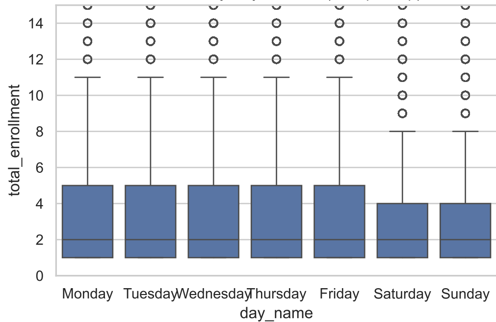
Enrollment by Day of Week (95th pct cap)
