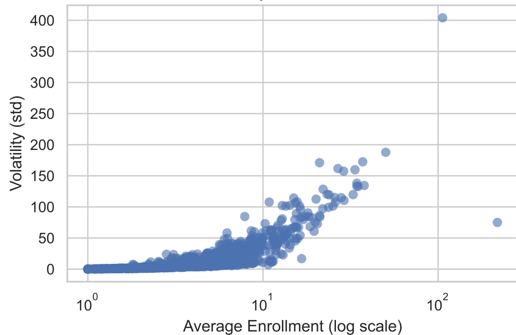
Volatility vs District Size
