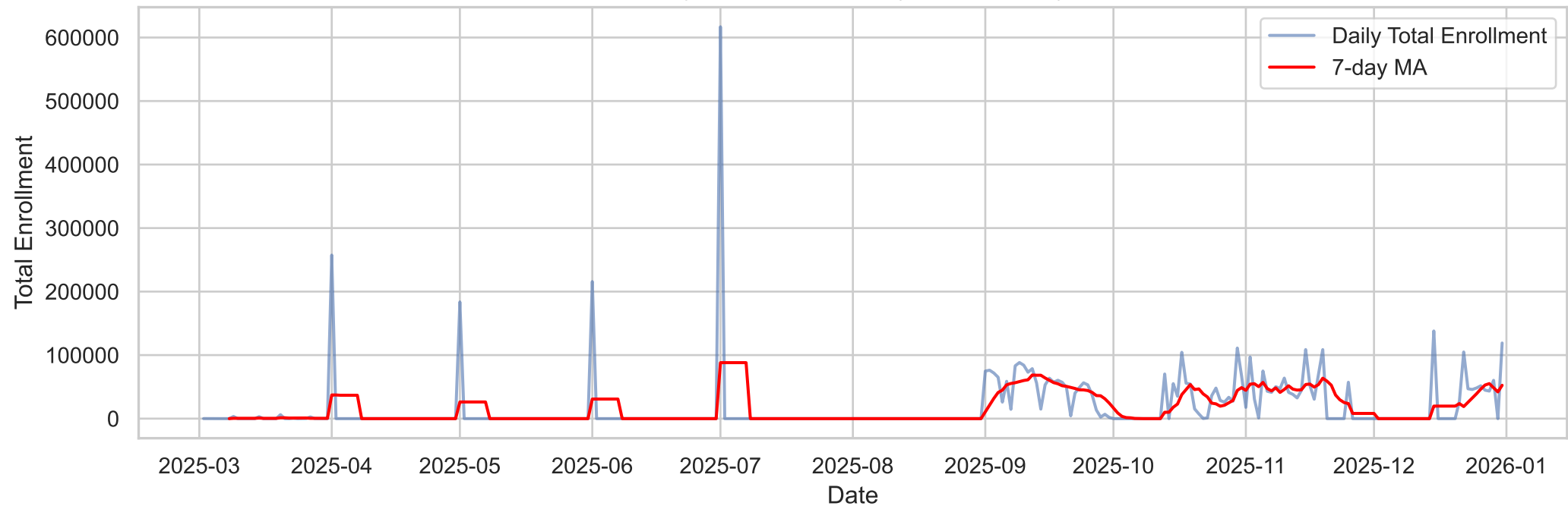
Daily Enrollment Trend (Mar-Dec 2025)
