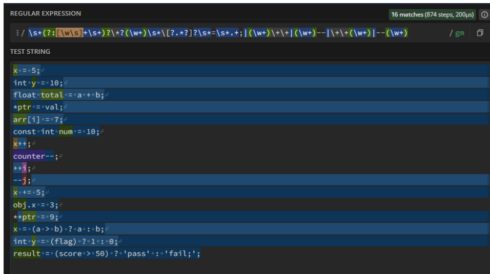
Figure 7.4: Example of the assignment statements our regex can match.
