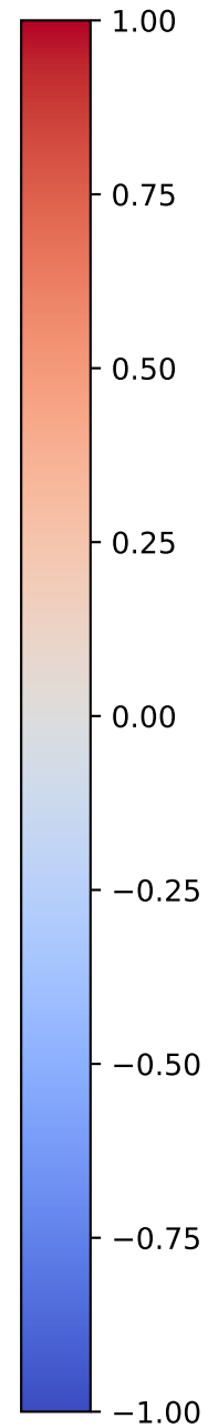
Llama-3.1-8B-Instruct: DRAT
