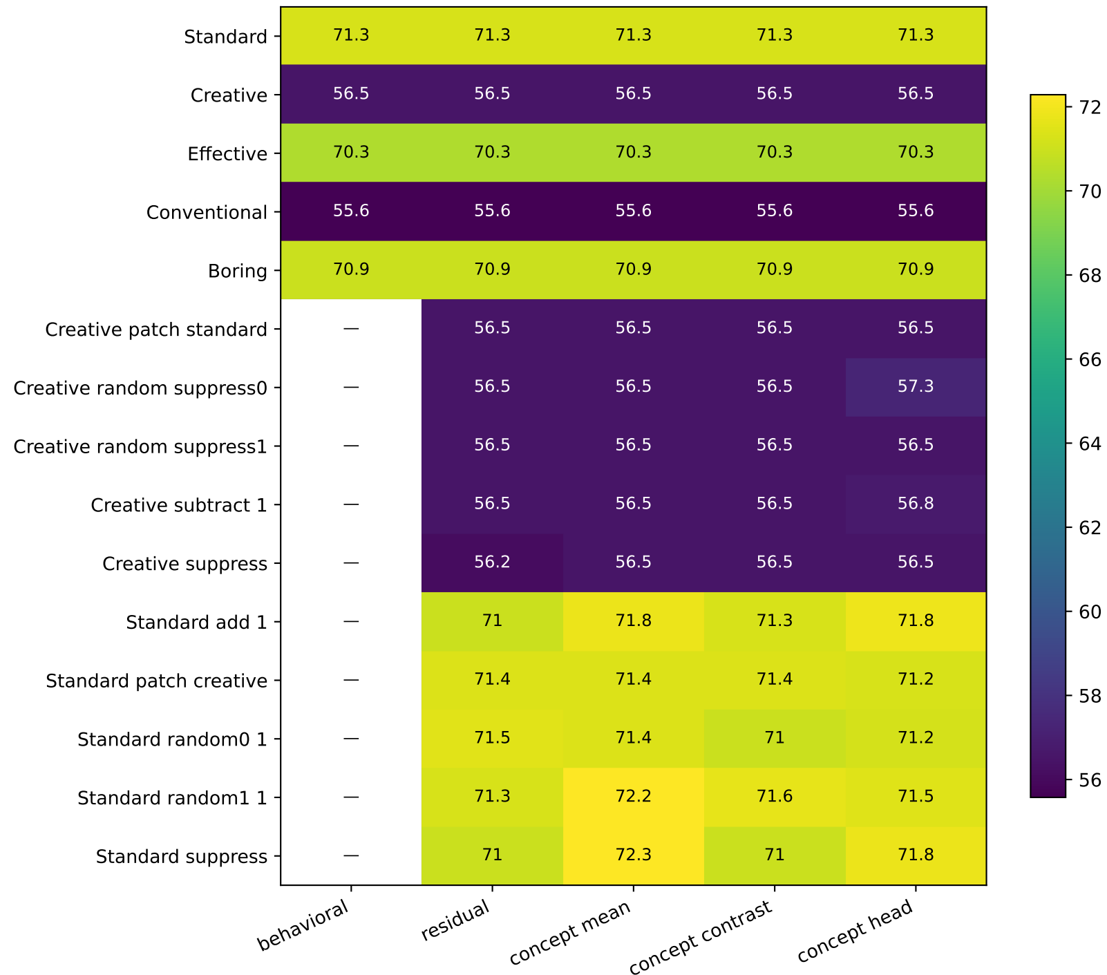
DRAT greedy: DRAT_Score
