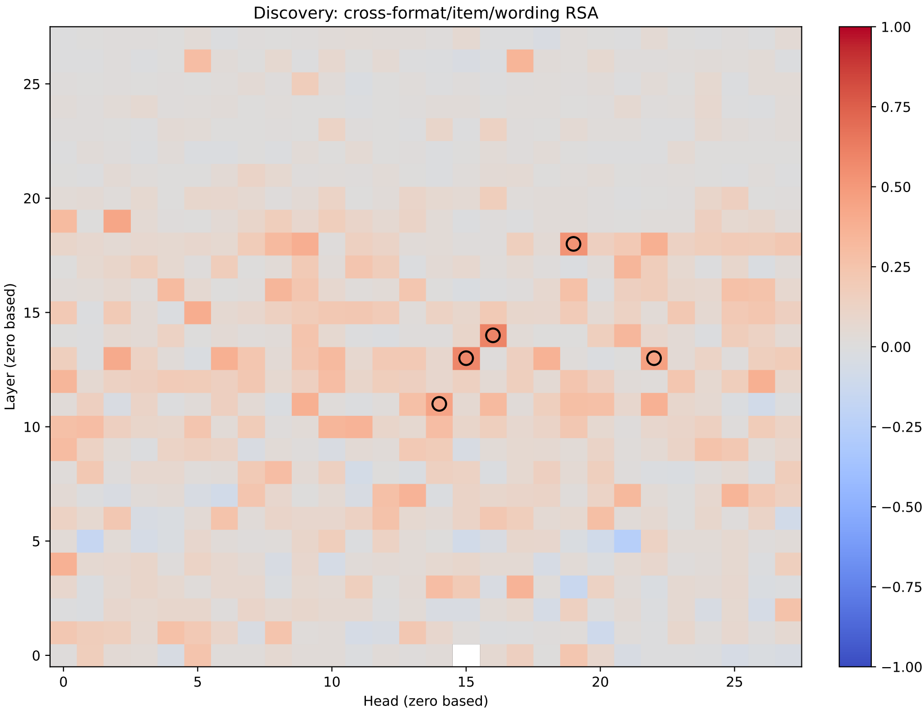
Qwen2.5-7B-Instruct: CDAT
