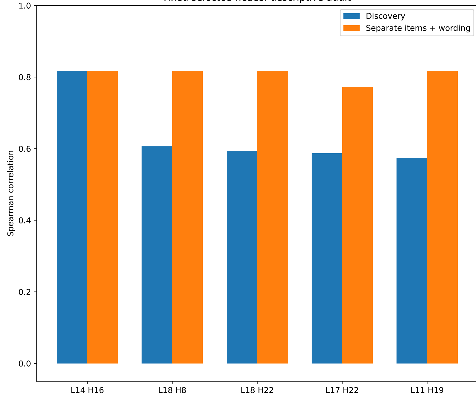
Fixed selected heads: descriptive audit
