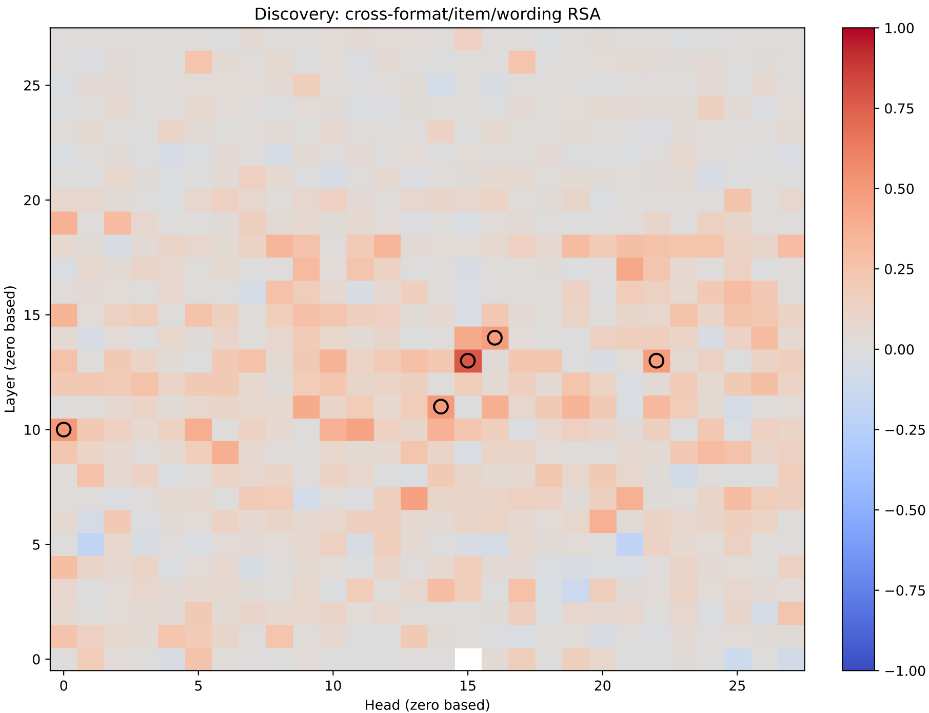
Qwen2.5-7B-Instruct: DRAT
