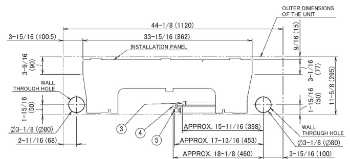
STANDARD LOCATION ON A WALL
