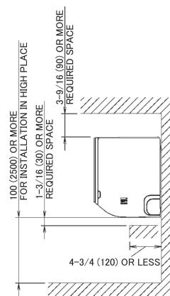
STANDARD LOCATION ON A WALL
