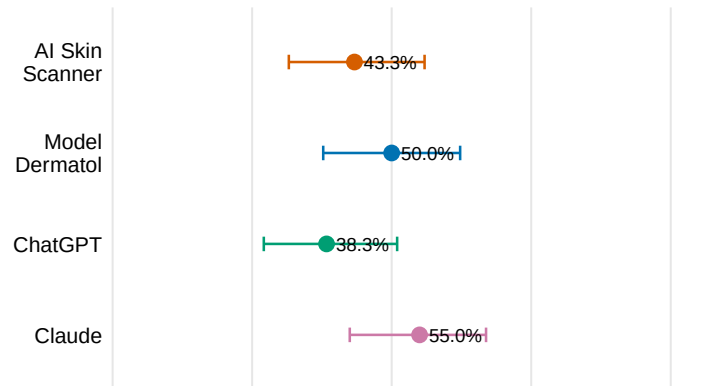
Melanoma spectrum
