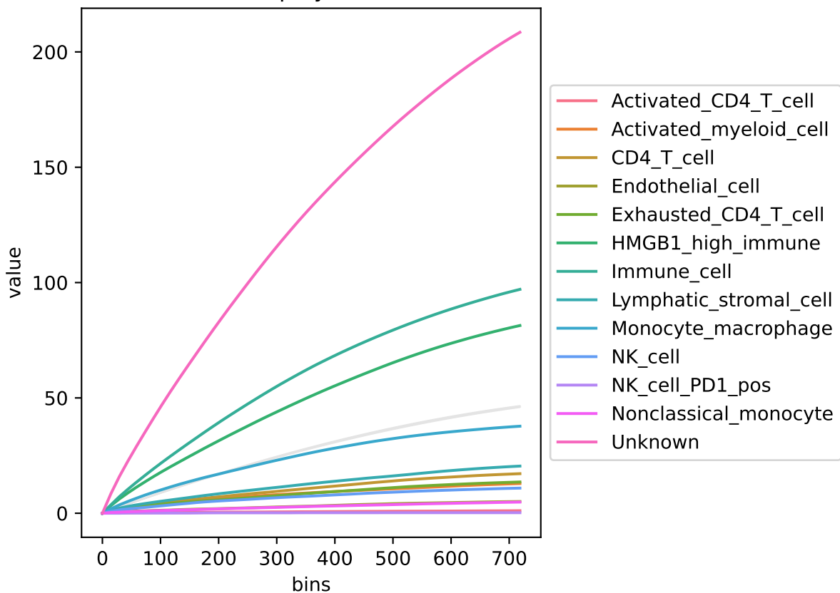
Ripley's L
